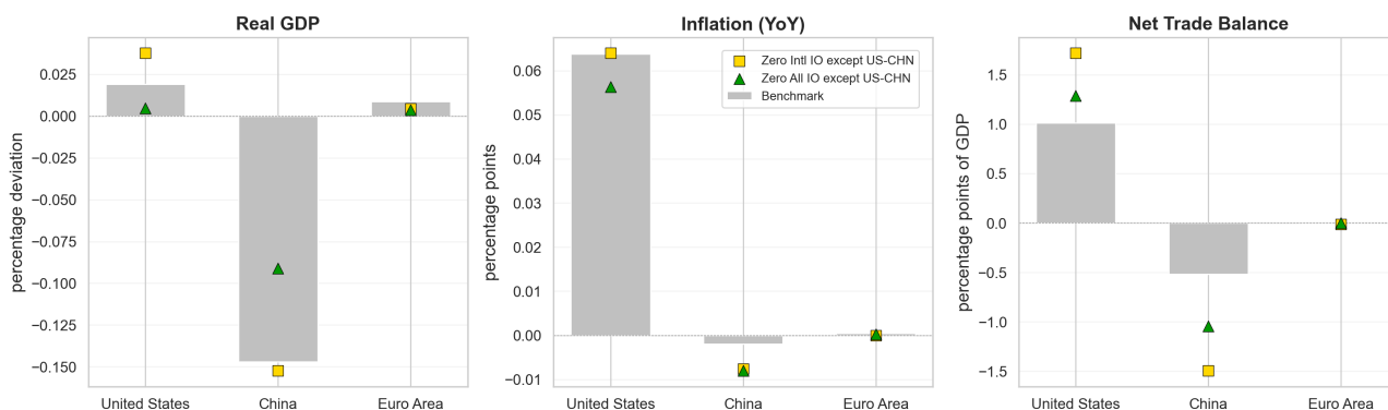
Figure 2: Production-Network Counterfactuals
