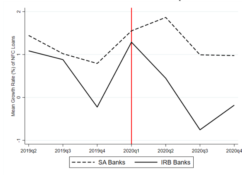
Figure 1: Credit exposures to Non Financial Corporations (NFC) at Bank Level. The two figures plot the average growth rate of the two lending measures (On-balance sheet exposures to NFCs in Panel A, and Loans to NFCs in Panel B), computed quarter by quarter, according to the two groups of banks. Source of data: FINREP. SA banks include banks reporting all corporate credit risk exposure using a Standardized Approach, IRB banks are banks in which a fraction of credit risk exposure is evaluated using Internal Ratings Based approach (source: COREP).
