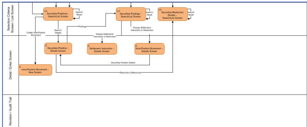
Illustration 6: Screen interrelation
