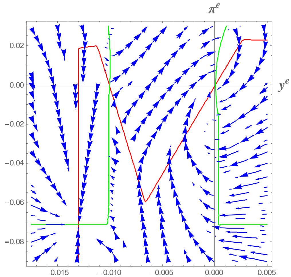
Figure 4: Learning stability dynamics with three steady states. Here y^e and \pi^e denote \hat{Y}^e and \hat{\pi}^e .
