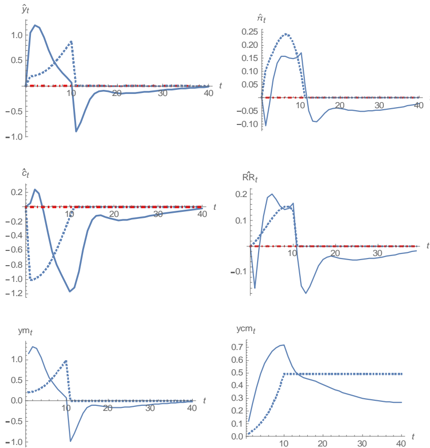
Figure 5: The upper panel shows the paths of output and inflation under RE (dotted line), learning (solid line) for a temporary policy change with T = 10 . The middle panel shows the paths of the corresponding consumption and ex ante one period real rate of interest ( \hat{R}_t - \hat{E}_t \pi_{t+1} ). The lower panel shows the distributed lag and cumulative output multipliers for the policy change. Here and in subsequent figures \hat{y}_t is used for \hat{Y}_t .
