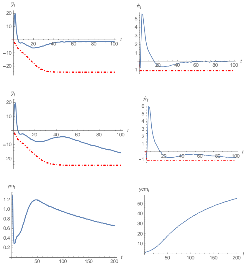
Figure 9: High discount factor, \beta = 0.995 . The top two panels show paths under learning with policy change (solid line) and without policy change (dashed line). Top panel: means of paths with eventual convergence to targeted steady state under policy. Middle panel: mean paths with eventual convergence to deflation trap despite policy. Bottom panel: distributed lag and cumulative output multipliers across all paths.
