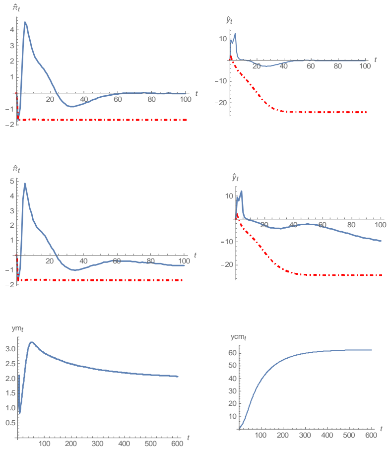
Figure 7: Large policy change. The top two panels show the paths of output and inflation under learning with policy change (solid line) and without policy change (dashed line) for T = 4 . Top panel: means of paths with convergence to targeted steady state under policy. Middle panel: means of paths with convergence to deflation trap despite policy. Bottom panel: distributed lag and cumulative output multipliers across all paths.
