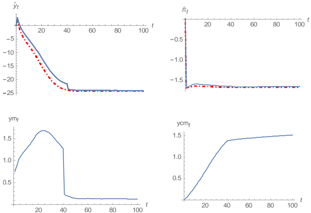
Figure 6: Small policy change. The upper panel shows the paths of output and inflation under learning with policy change (solid line) and learning without policy change (dashed line) for a temporary policy change with T = 40 . The lower panel shows the distributed lag and cumulative output multipliers for the policy change.
