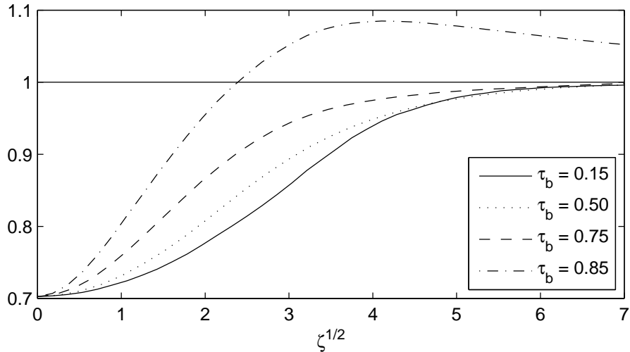
Figure 5: Relative MSFE of forecast combination and post-break sample forecasts
