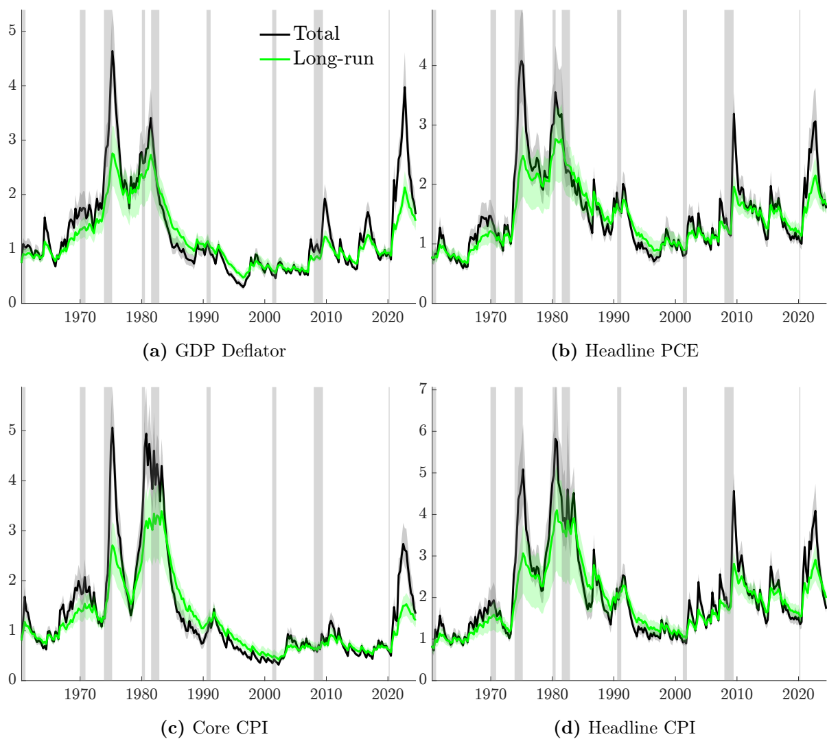
Figure D3: Estimated volatility for different inflation measures
