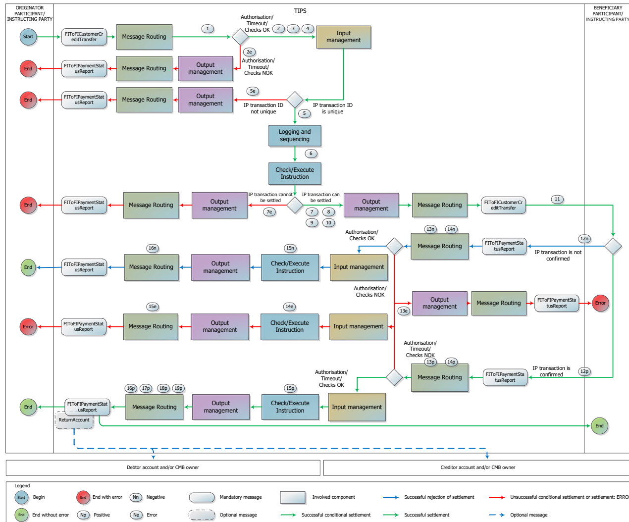
Figure 17 – Instant Payment transaction flow
