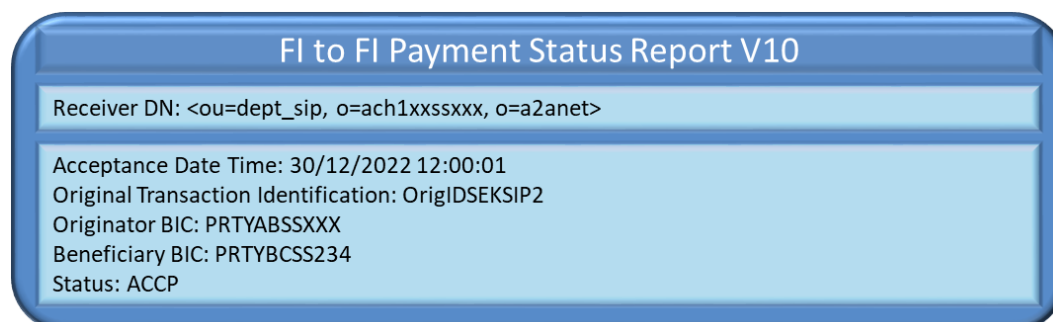
Figure 105 – Instant Payment transaction SIP settlement model successful scenario - non-Euro currency - FltoFIPaymentStatusReportV10
