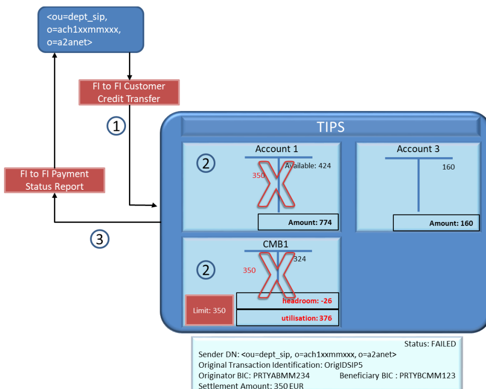
Figure 107 – Headroom error transaction failed
