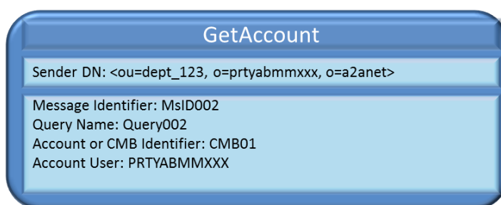
Figure 166 – Successful Get Account
