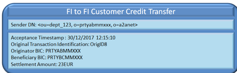
Figure 47 – Delayed Beneficiary-side answer FItoFICustomerCreditTransfer
