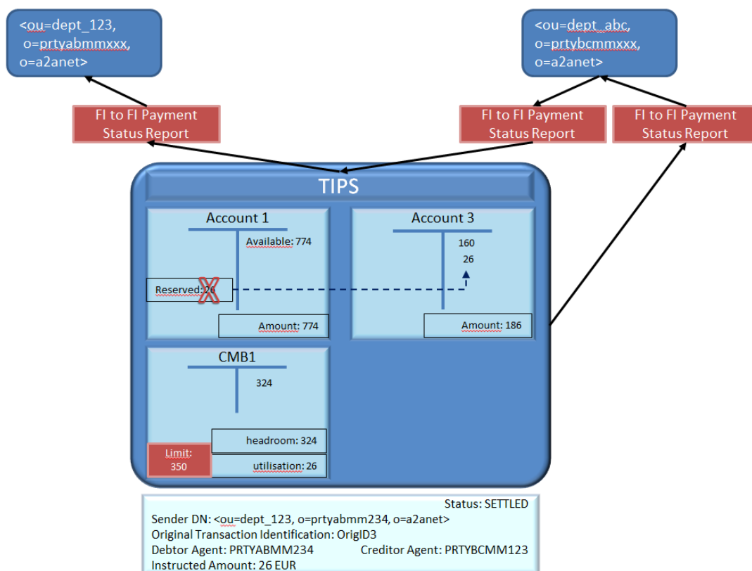
Figure 27 – Instant Payment transaction successful scenario settlement
