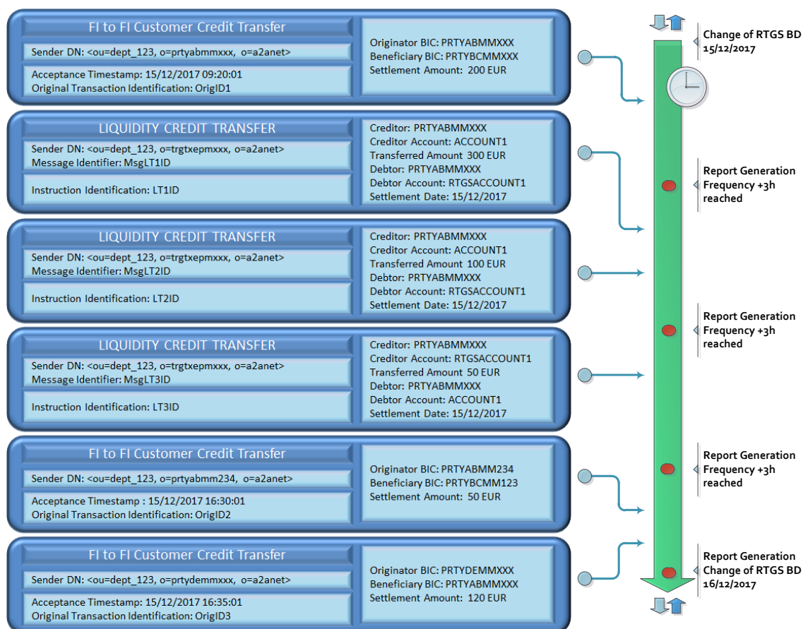
Figure 182 – Statement of Accounts example: list of transaction (delta mode)
