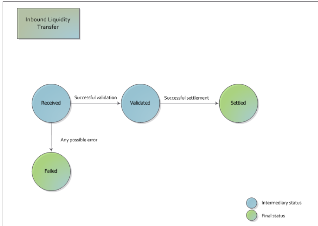
Figure 10 – Inbound Liquidity Transfer status
