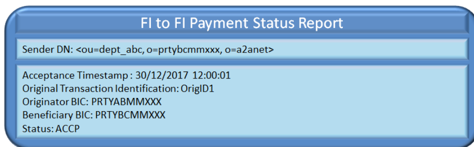
Figure 22 – Instant Payment transaction successful scenario FItoFIPaymentStatusReport
