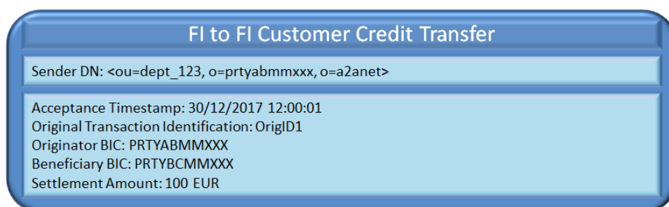
Figure 20 – Instant Payment transaction successful scenario FltoFICustomerCreditTransfer
