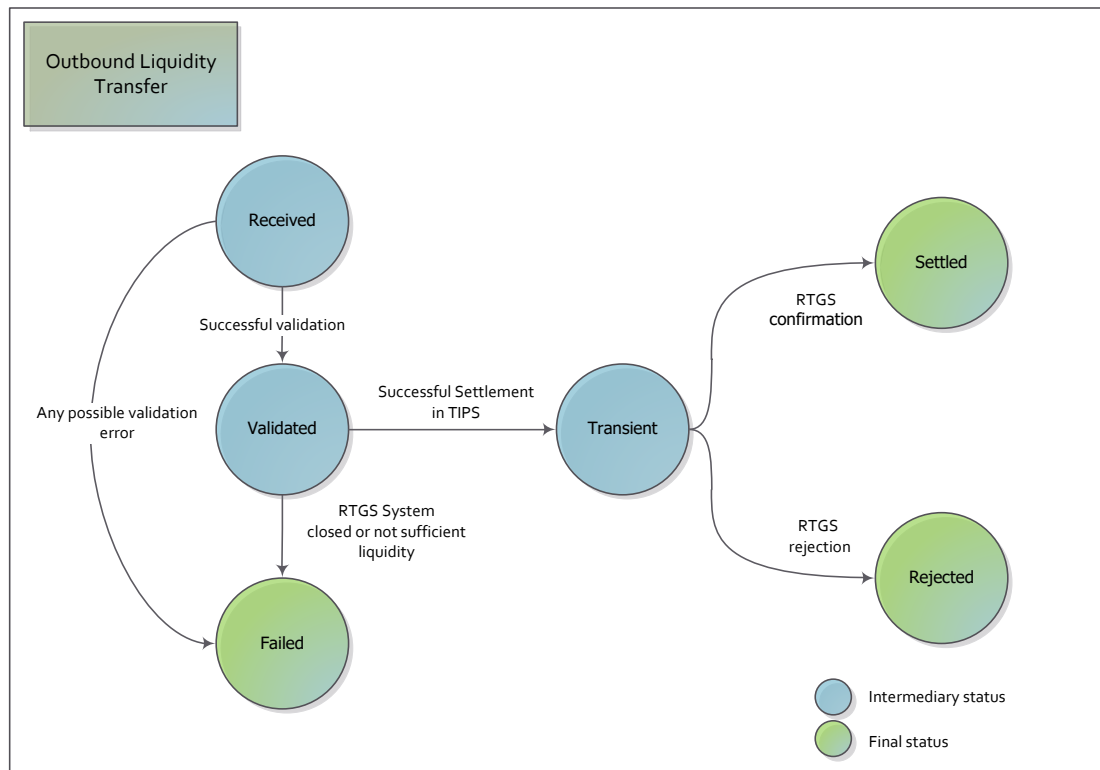
Figure 11 – Outbound Liquidity Transfer status
