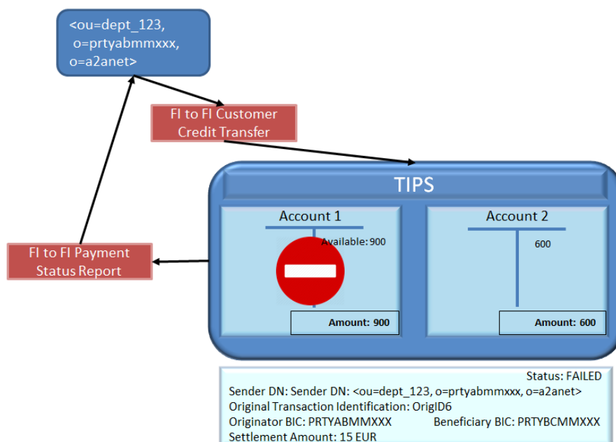
Figure 40 – Blocked account error transaction failed
