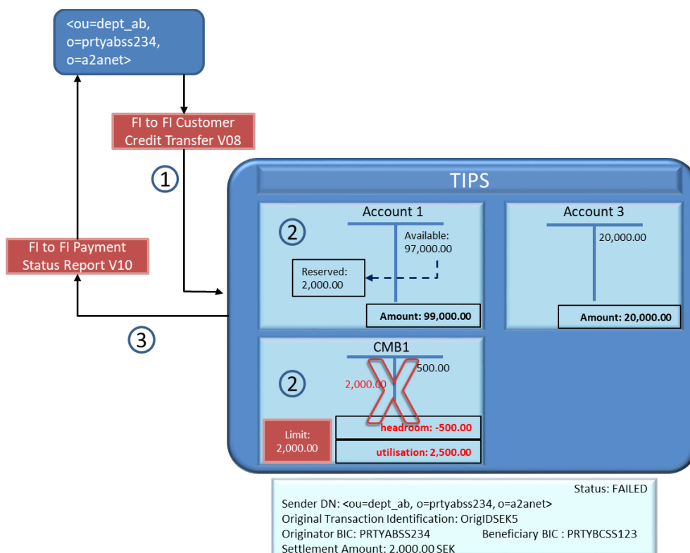
Figure 74 – Headroom error transaction failed
