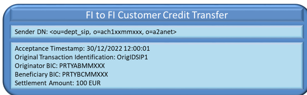
Figure 94 – Instant Payment transaction SIP settlement model successful scenario - Euro currency - FltoFICustomerCreditTransfer
