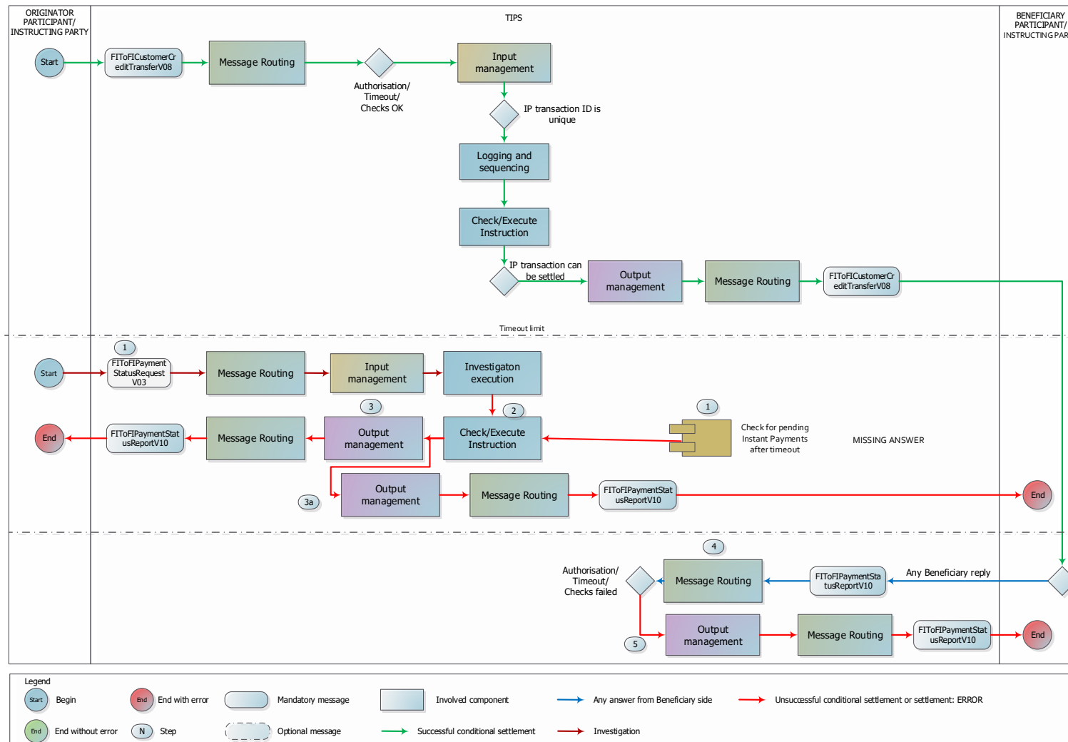
Figure 55 – Instant Payment transaction missing/delayed Beneficiary-side answer flow (non-Euro currencies)
