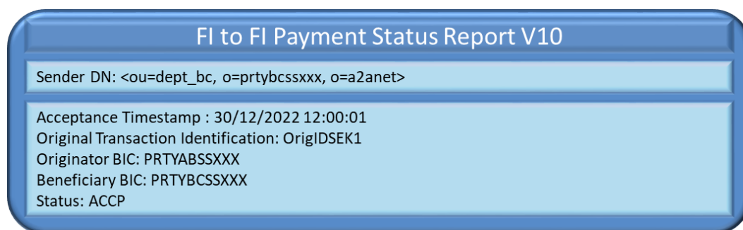
Figure 59 – Instant Payment transaction successful scenario FItoFIPaymentStatusReportV10
