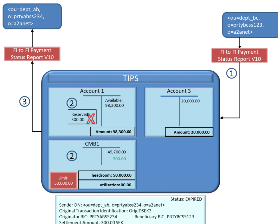
Figure 82 – Beneficiary side timeout error un-reservation release
