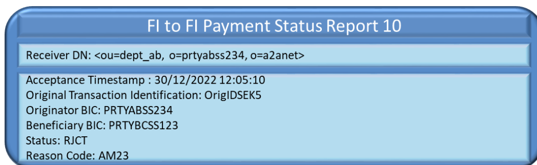
Figure 75 – Headroom error FItoFIPaymentStatusReportV10
