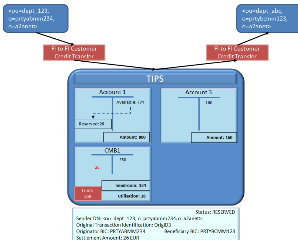
Figure 25 – Instant Payment transaction successful scenario reservation
