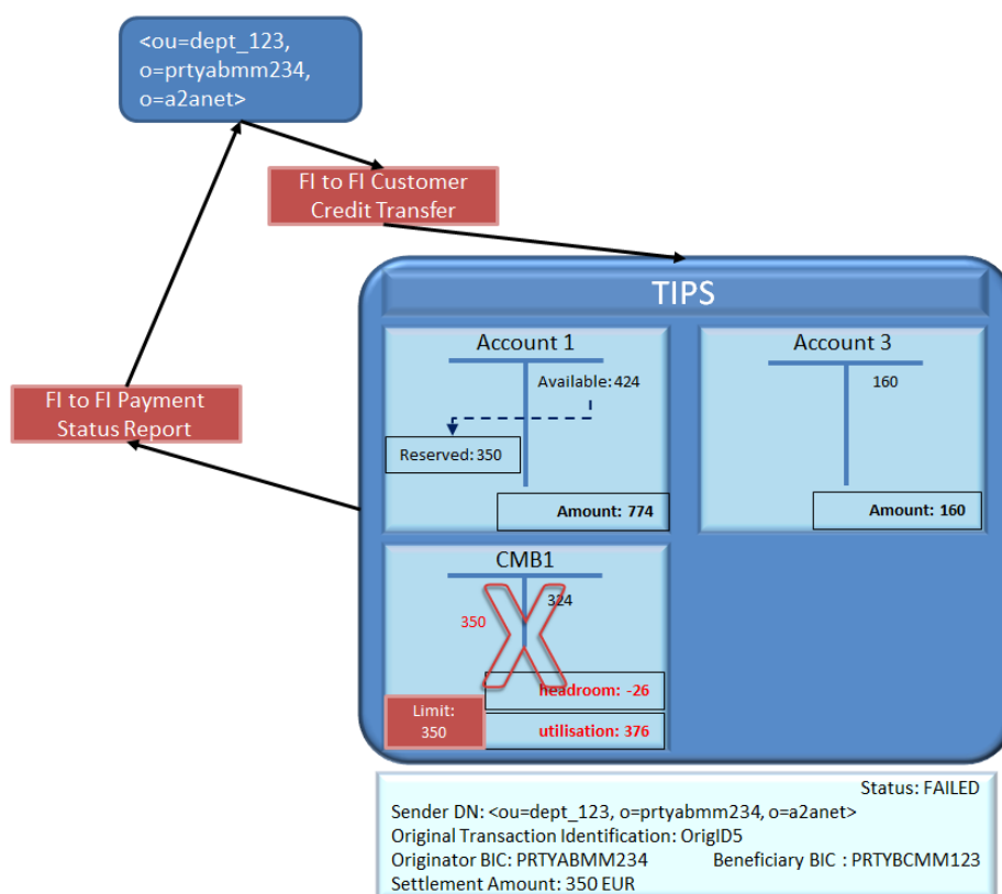
Figure 37 – Headroom error transaction failed
