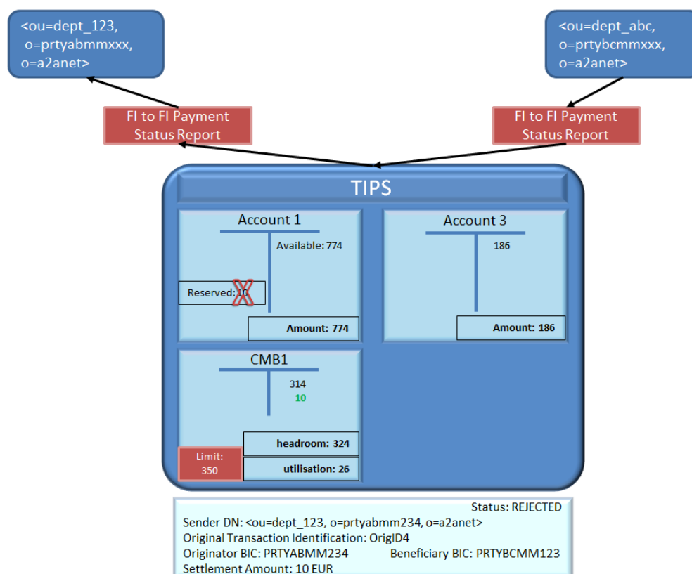
Figure 35 – Instant Payment transaction rejected order unreservationrelease
