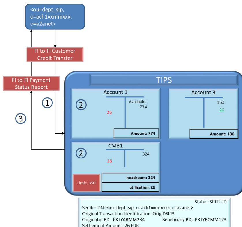
Figure 98 – Instant Payment transaction SIP settlement model successful scenario
