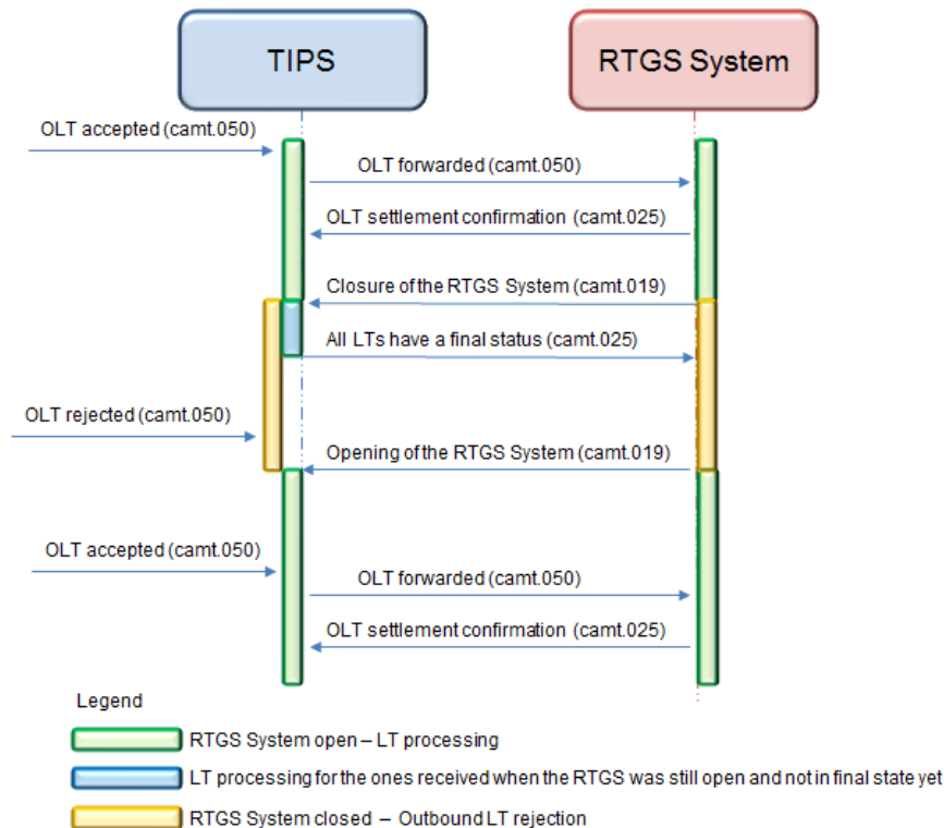
Figure 13 – Closure and opening of the RTGS System
