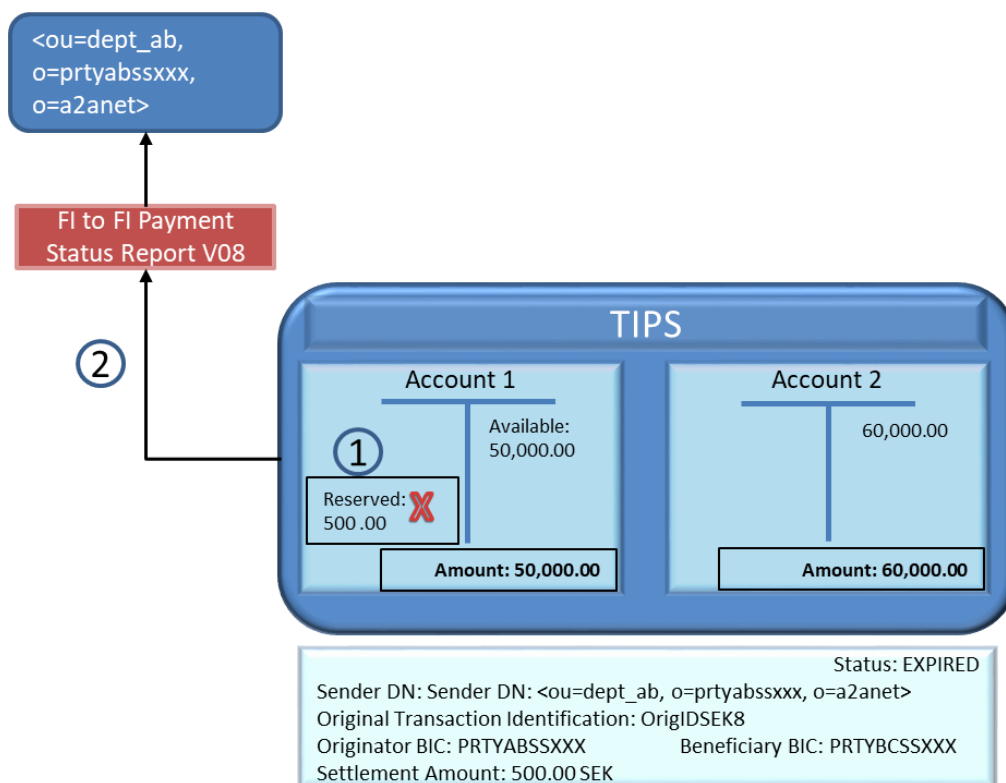
Figure 86 – Delayed Beneficiary-side answer un-reservation
