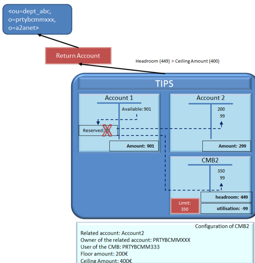
Figure 160 – Ceiling notification settlement
