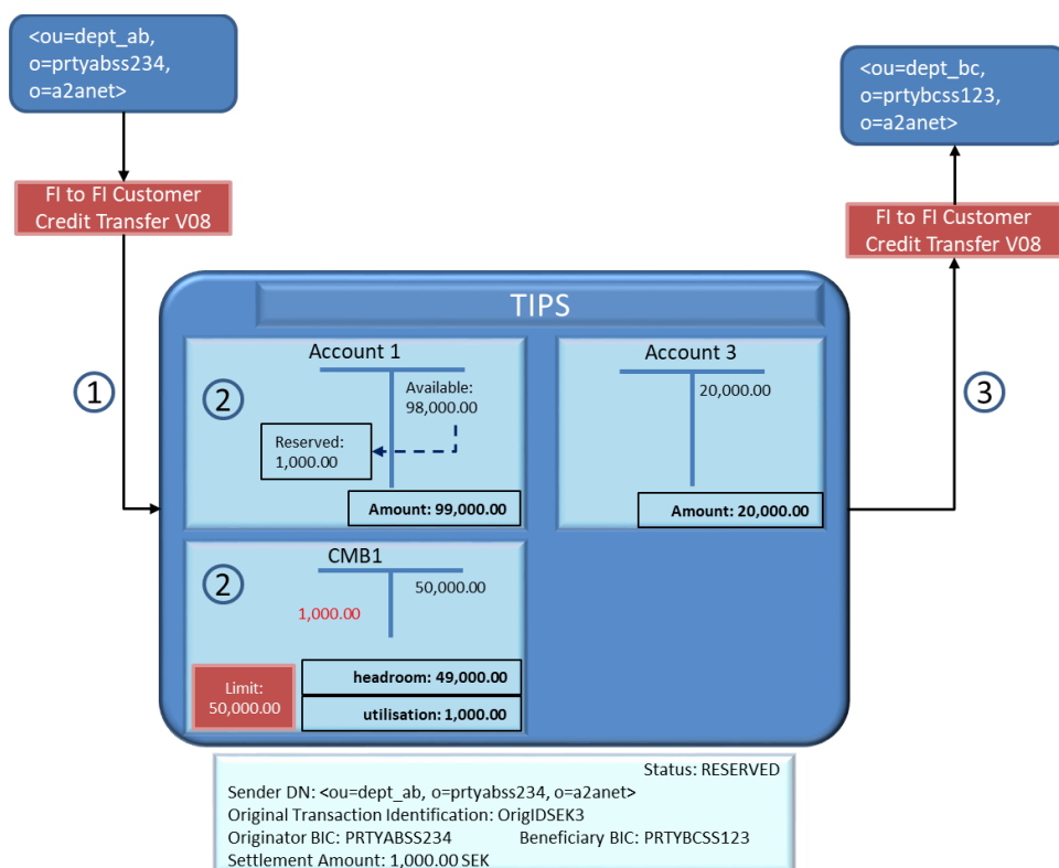
Figure 62 – Instant Payment transaction successful scenario reservation
