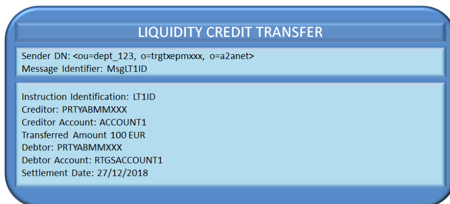
Figure 133 – Successful Inbound Liquidity Transfer order: liquidity credit transfer
