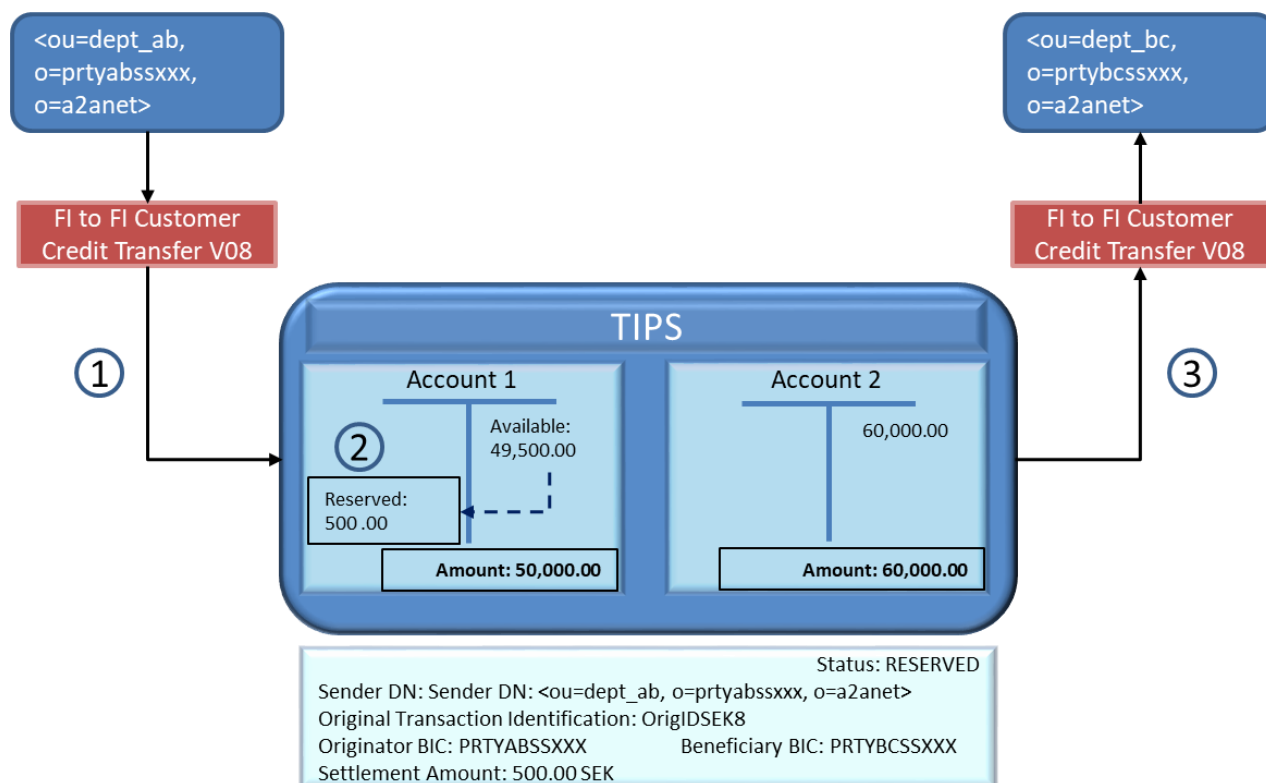
Figure 85 – Delayed Beneficiary-side answer reservation
