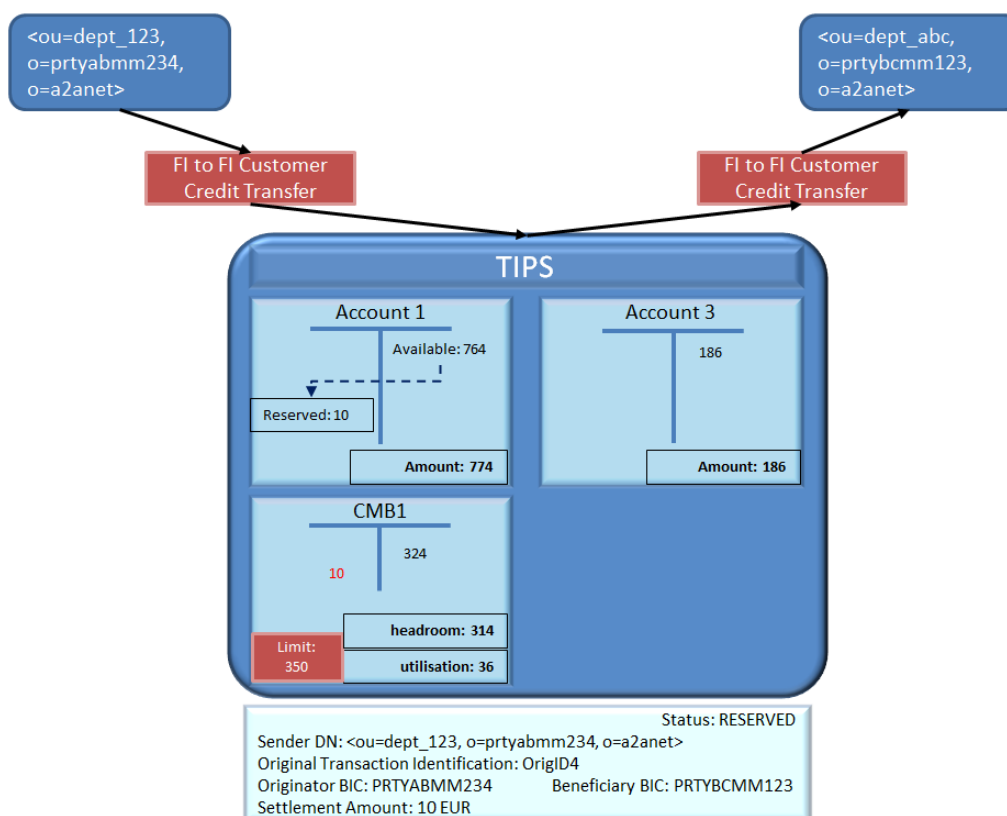
Figure 33 – Instant Payment transaction rejected order reservation
