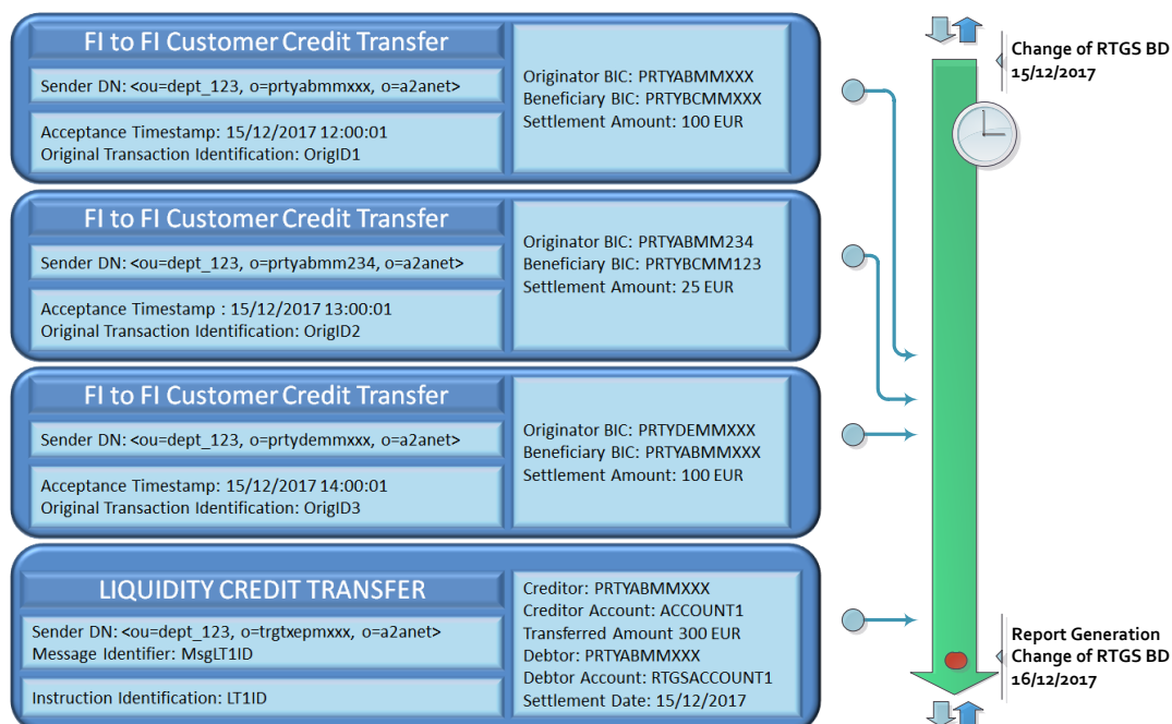
Figure 174 – Statement of Account Turnover example: list of transactions
