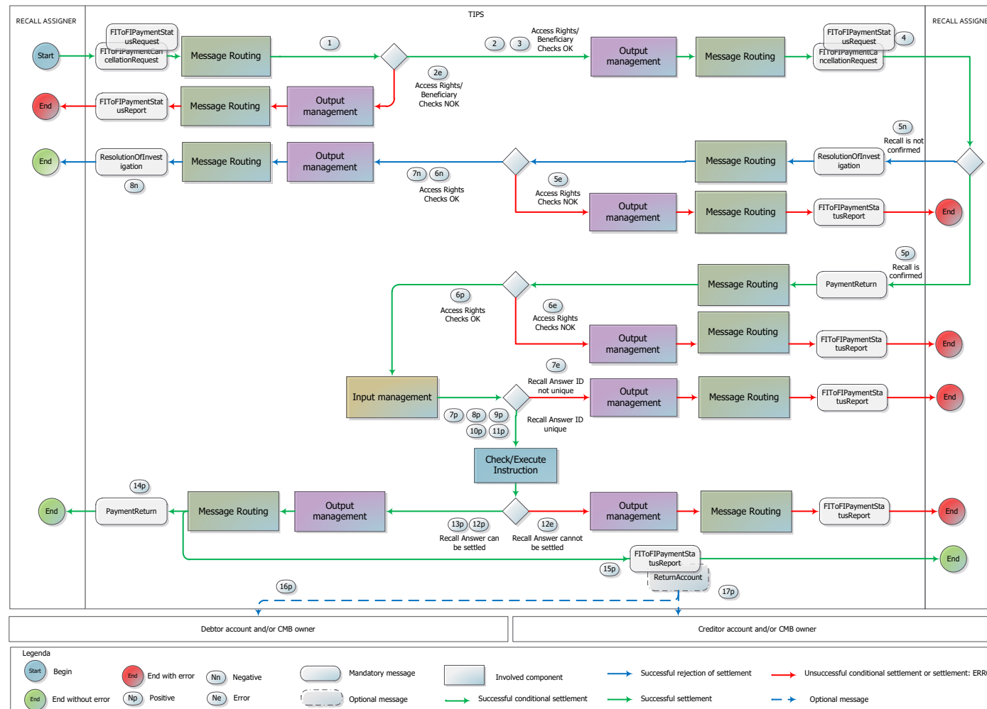
Figure 52 – Recall flow
