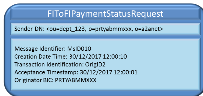
Figure 69 – Unsuccessful FIToFIPaymentStatusRequest
