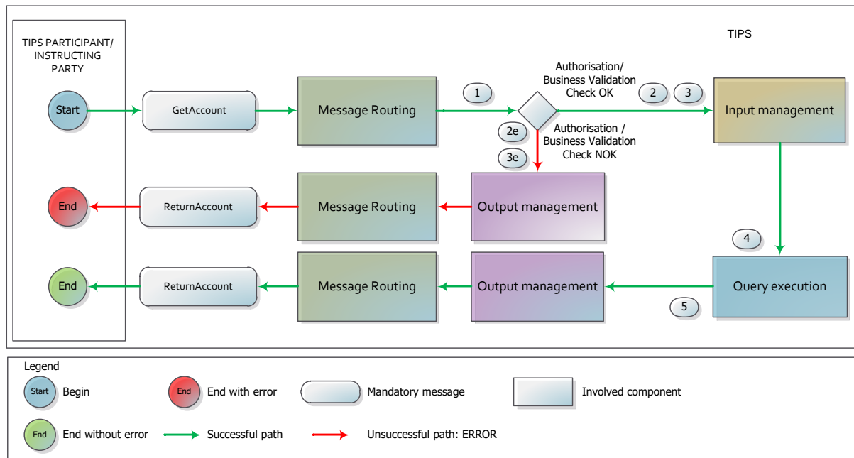
Figure 102 – Account Balance Status query flow
