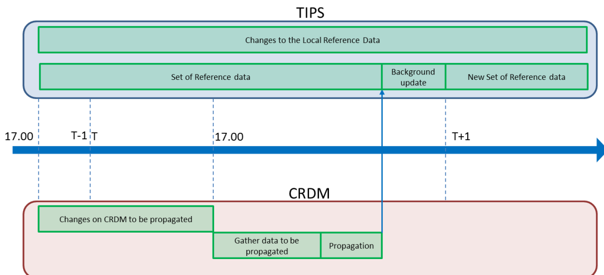
Figure 13 – Interaction between CRDM and TIPS 14
