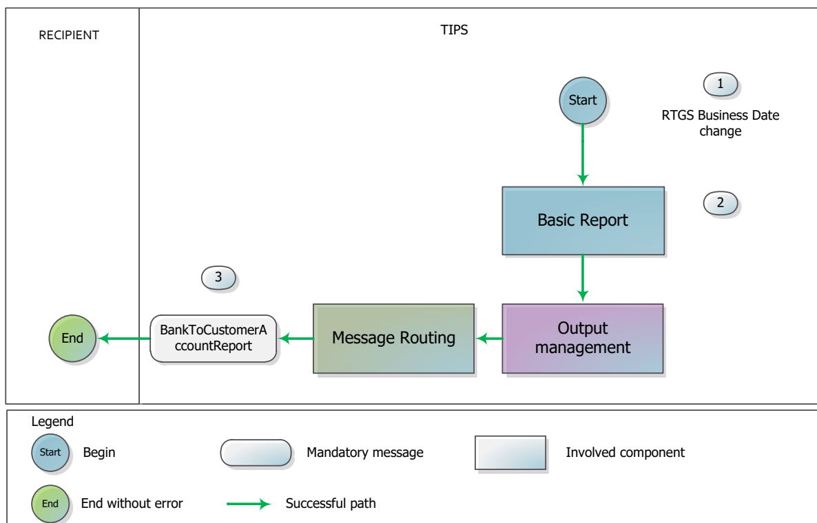
Figure 111 – Statement of Account Turnover flow
