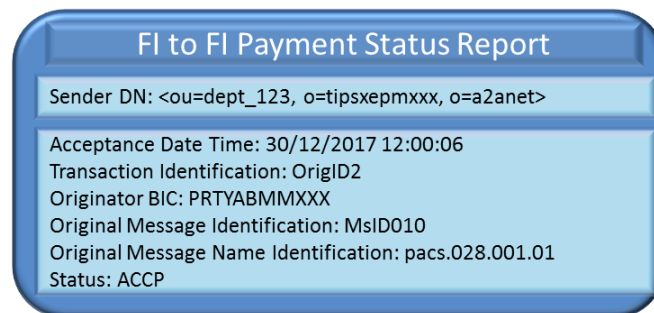
Figure 68 – Successful FIToFIPaymentStatusReport
