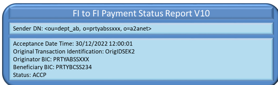
Figure 72 – Successful Instant Payment transaction: FIToFIPaymentStatusReportV10
