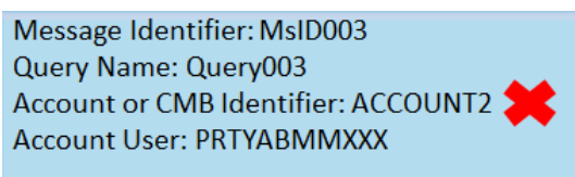
Figure 191 – Unsuccessful GetAccount: account retrieval failure
