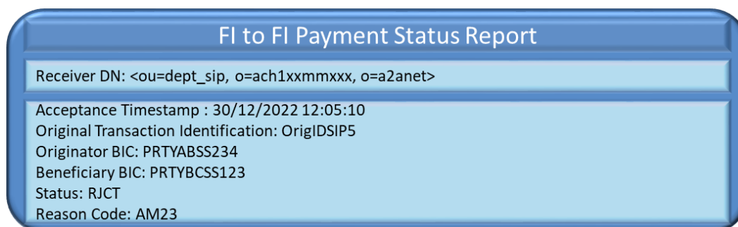
Figure 113 – Headroom error: FItoFIPaymentStatusReport
