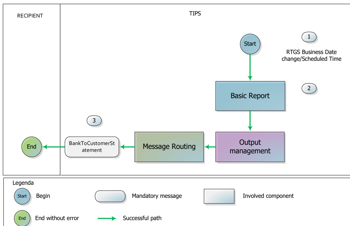
Figure 203 – Statement of Accounts flow
