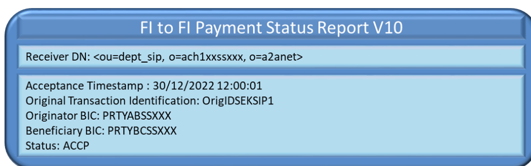
Figure 107 – Successful Instant Payment in non-Euro currency with SIP: FittoFIPaymentStatusReportV10
