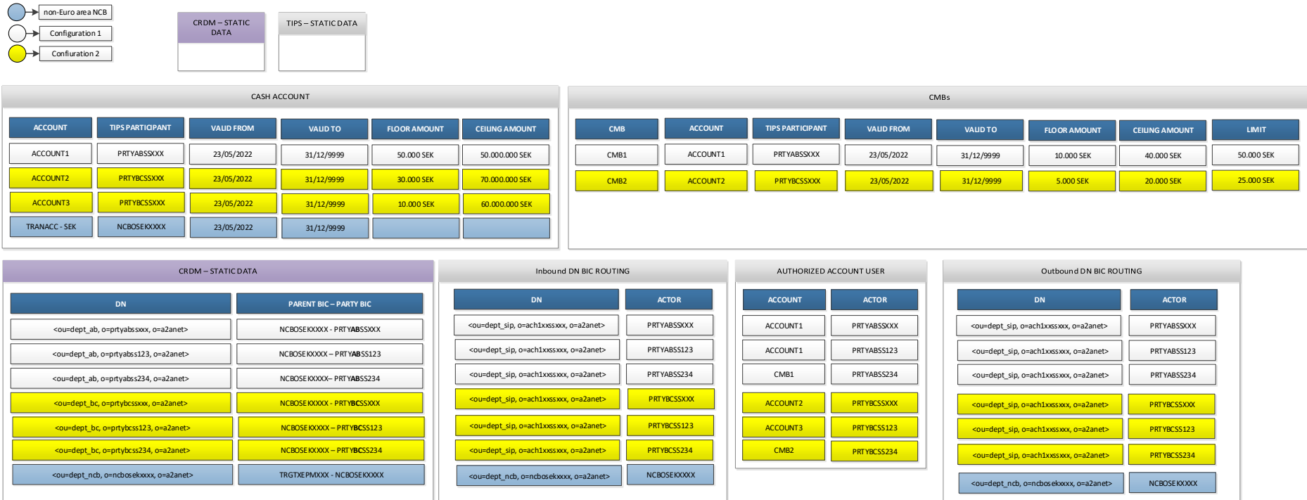
Figure 98 – Instant Payment transaction in a non-Euro currency - SIP settlement model - examples data constellation
