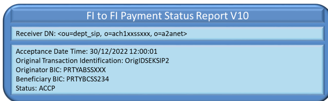
Figure 110 – Successful Instant Payment in non-Euro currency with SIP: FItoFIPaymentStatusReportV10
