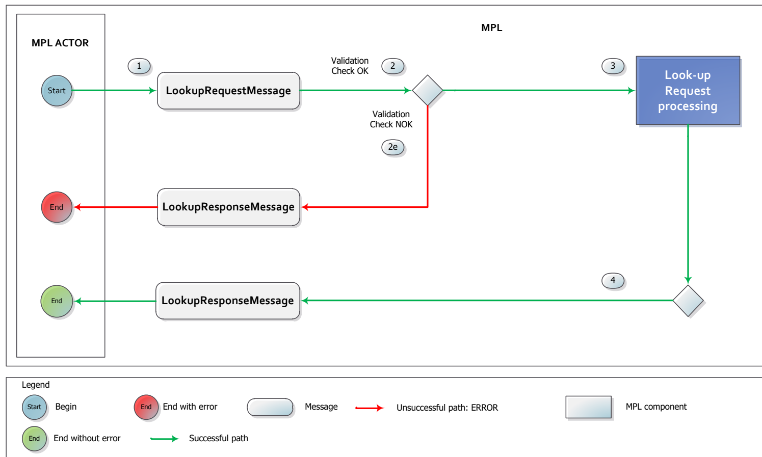
Figure 5 – Look-Up process
