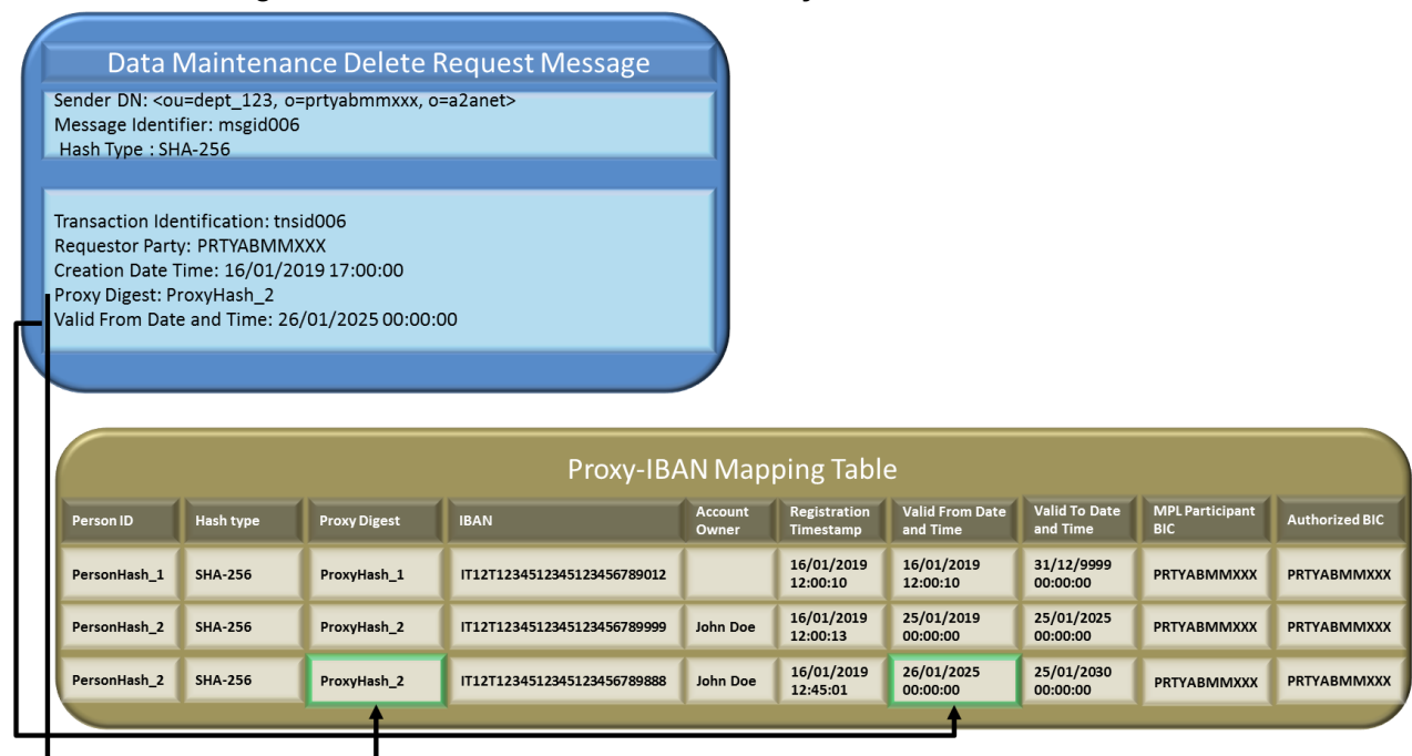
Figure 46 – Successful scenario 6 – Proxy-IBAN existence Check
