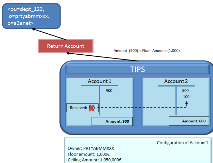
Figure 9796 – Floor notification settlement
