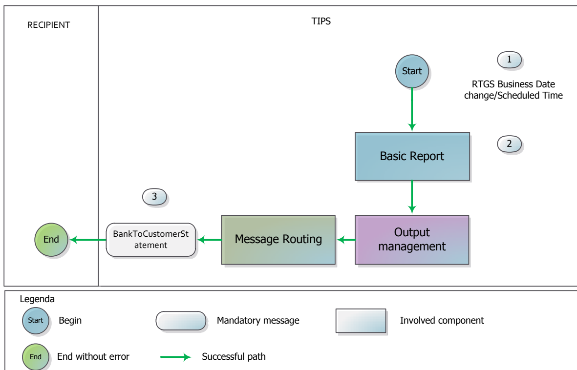
Figure 115114 – Statement of Accounts flow
