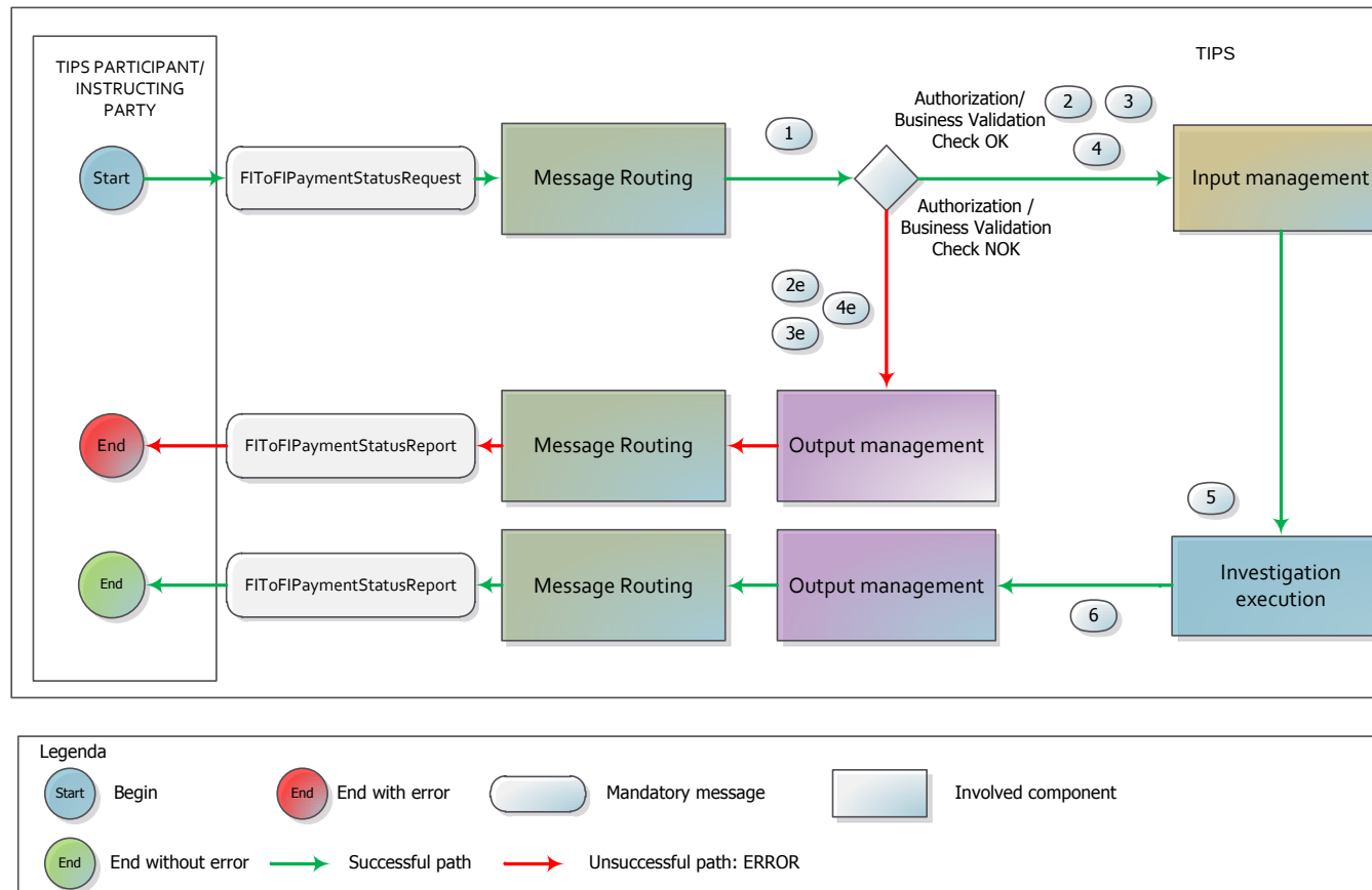
Figure 6564 – Investigation Flow
