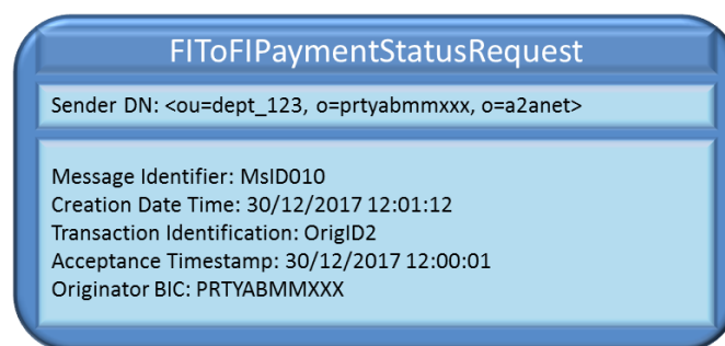
Figure 6766 – Successful FIToFIPaymentStatusRequest
