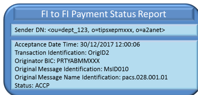
Figure 6867 – Successful FIToFIPaymentStatusReport
