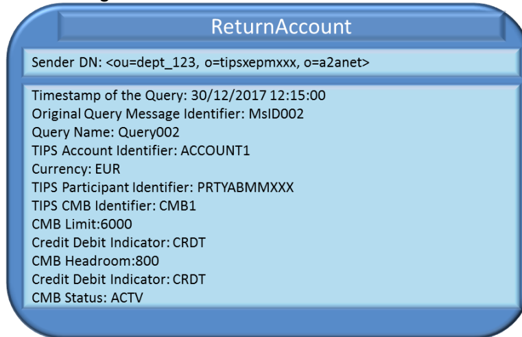
Figure 106105 - Successful ReturnAccount
