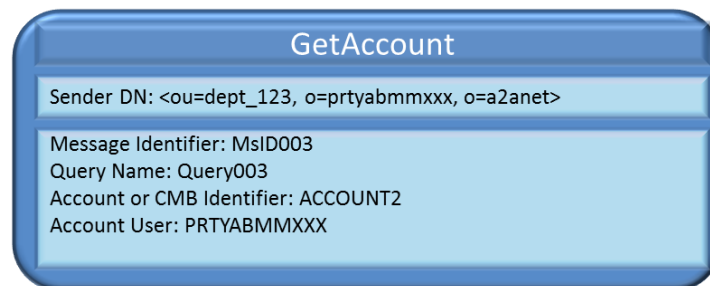
Figure 107106 – Unsuccessful GetAccount
