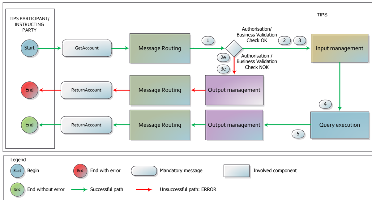
Figure 101100 – Account Balance Status query flow
