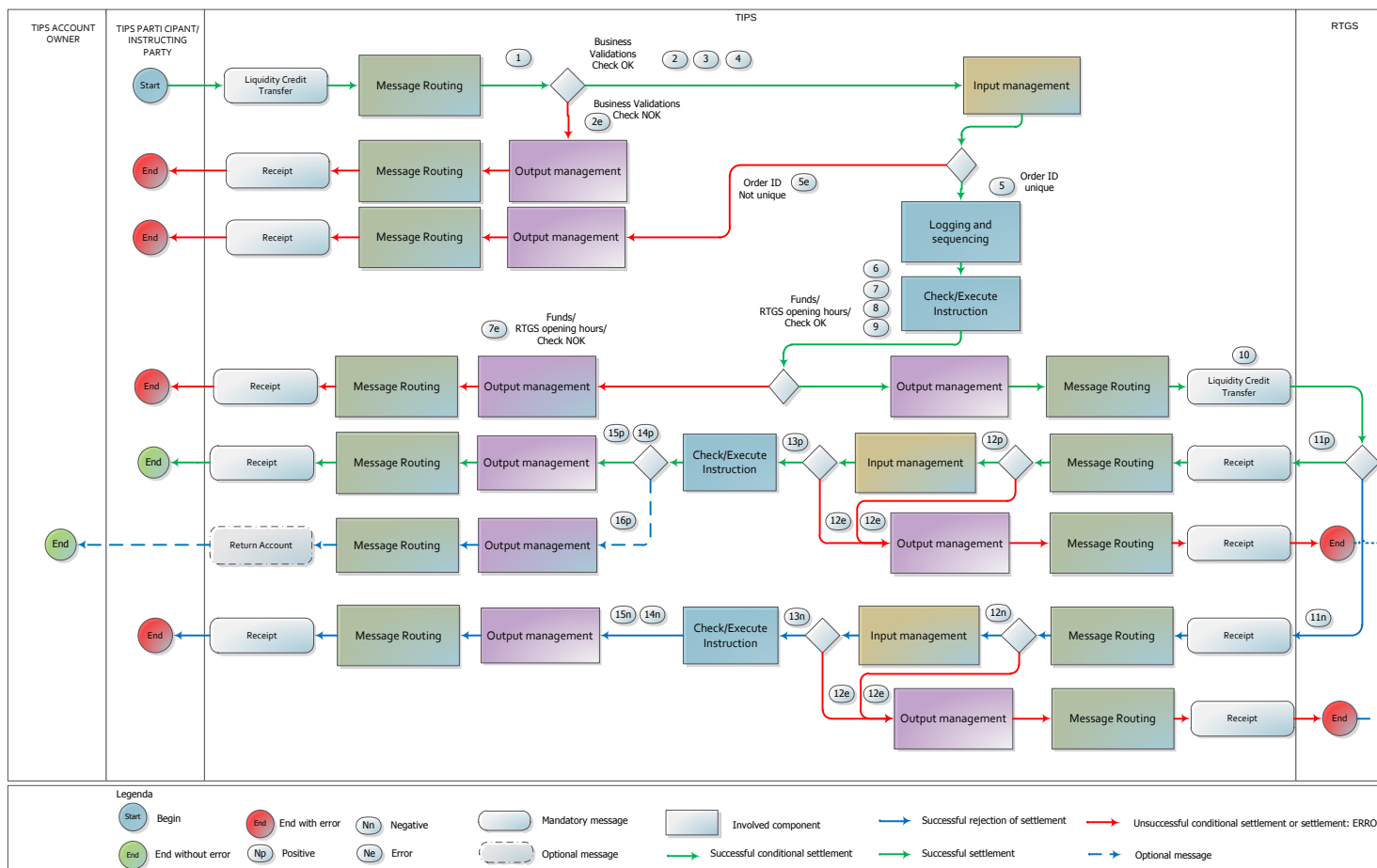
Figure 8079 – Outbound Liquidity Transfer Order flow
