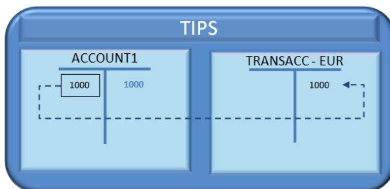
Figure 8382 – Successful Outbound Liquidity Transfer order settlement
