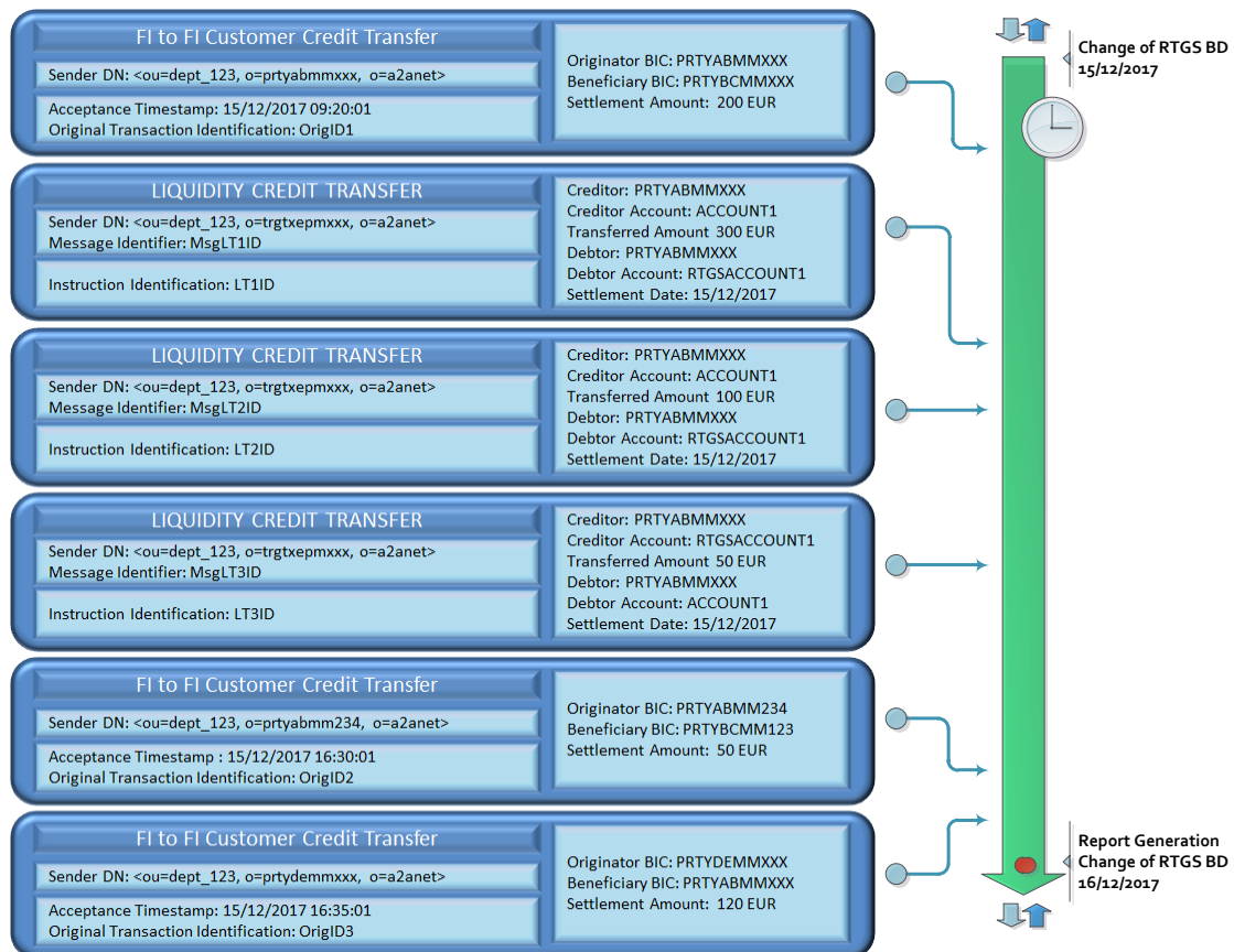
Figure 119118 – Statement of Accounts example: list of transactions (full mode)
