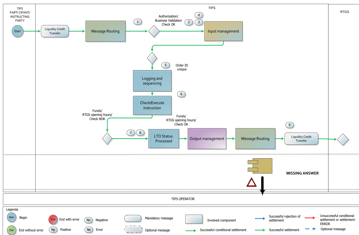
Figure 9594 – Outbound Liquidity Transfer: Missing RTGS answer flow
