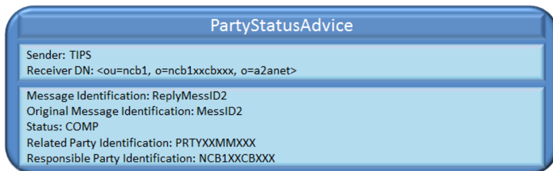
Figure 133132 – Unblock of a TIPS Participant successful scenario: PartyStatusAdvice
