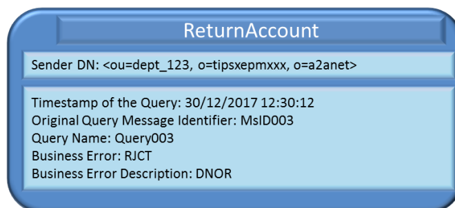
Figure 109108 – Unsuccessful ReturnAccount
