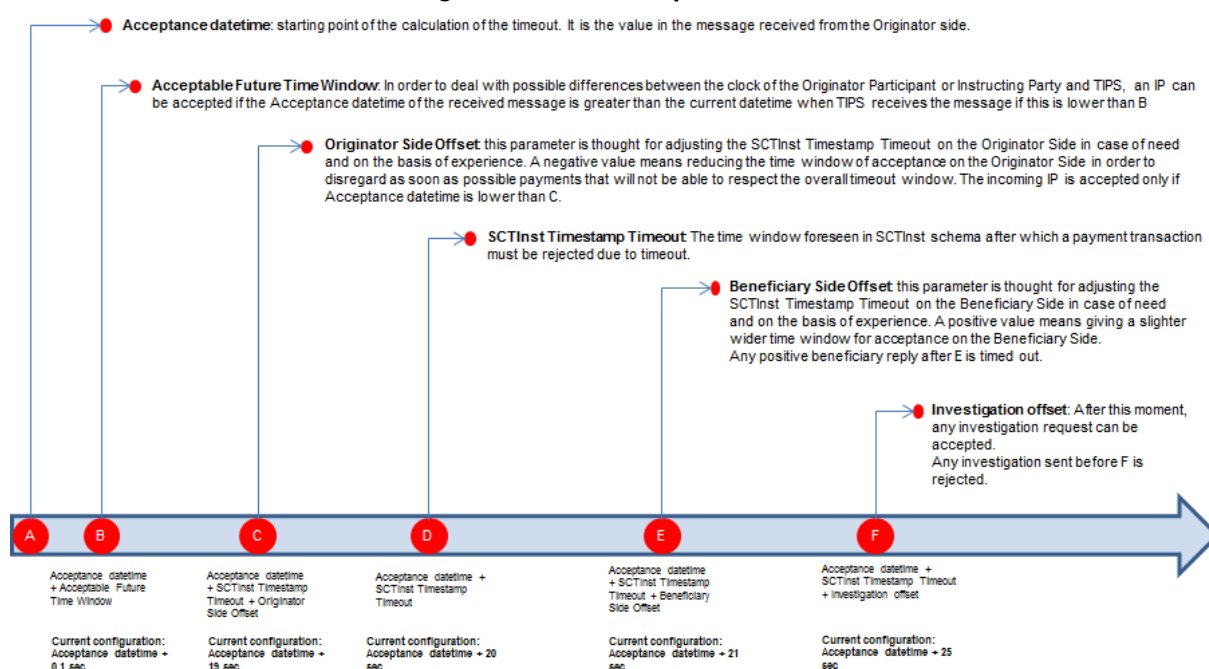
Figure 14 – Timeout parameters
