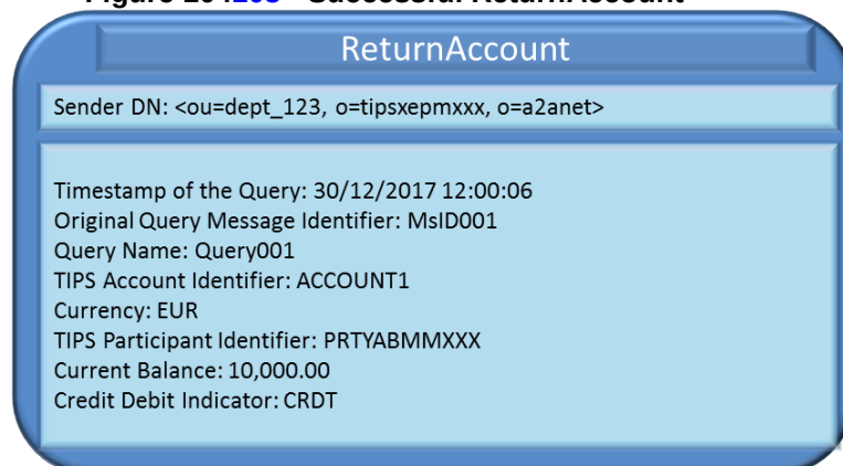
Figure 104103 - Successful ReturnAccount
