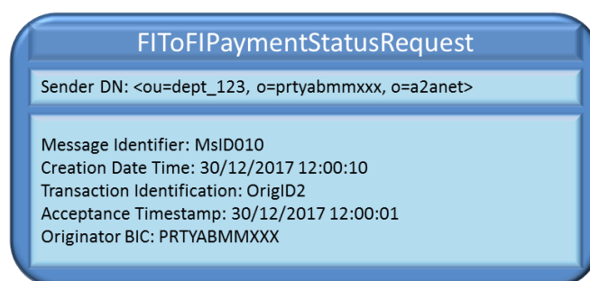
Figure 6968 – Unsuccessful FIToFIPaymentStatusRequest
