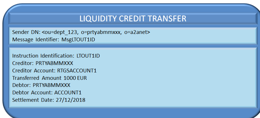
Figure 8281 – Successful Outbound Liquidity Transfer order: Liquidity Credit Transfer
