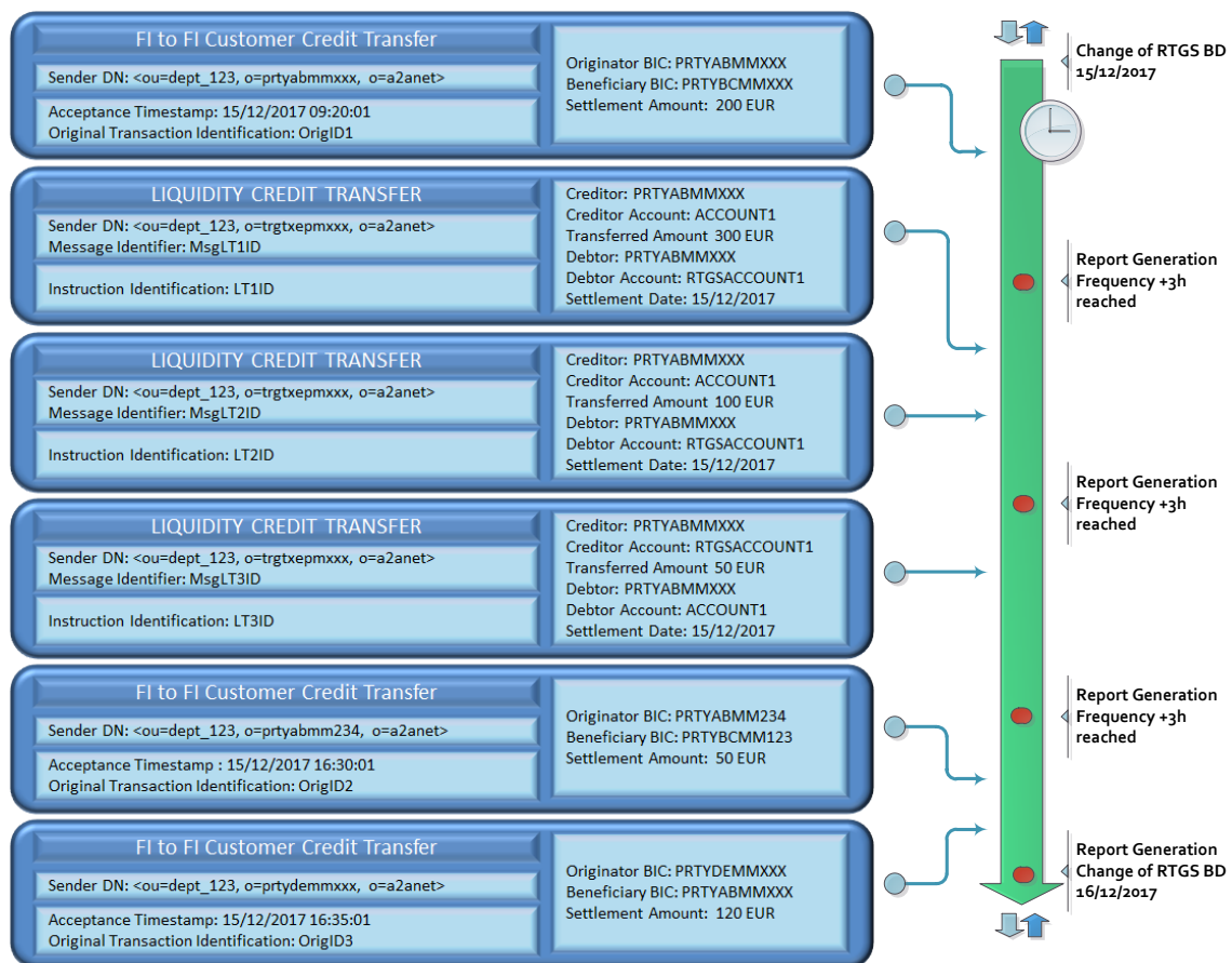
Figure 121120 – Statement of Accounts example: list of transaction (delta mode)
