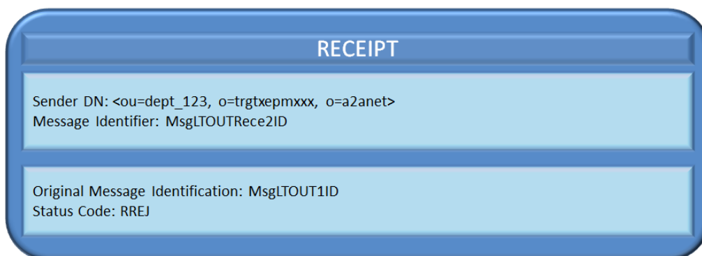
Figure 9291 – Outbound Liquidity Transfer order: negative Receipt sent by the RTGS
