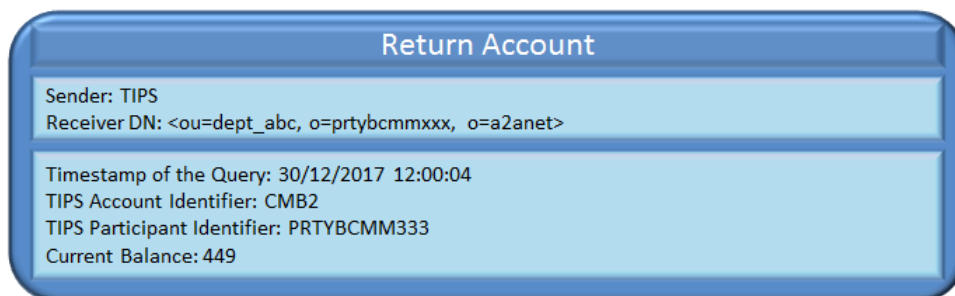
Figure 10099 – Ceiling notification ReturnAccount
