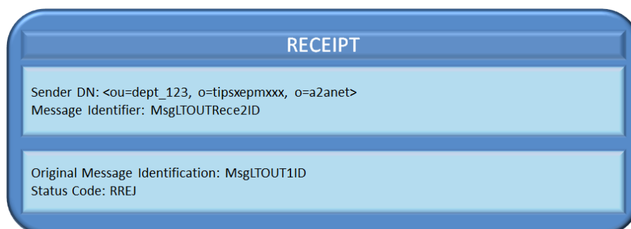
Figure 9493 – Outbound Liquidity Transfer order: negative Receipt sent by TIPS
