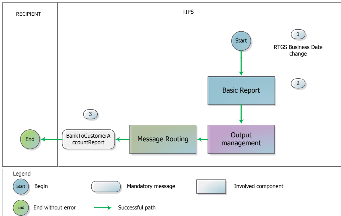
Figure 110109 – Statement of Account Turnover flow
