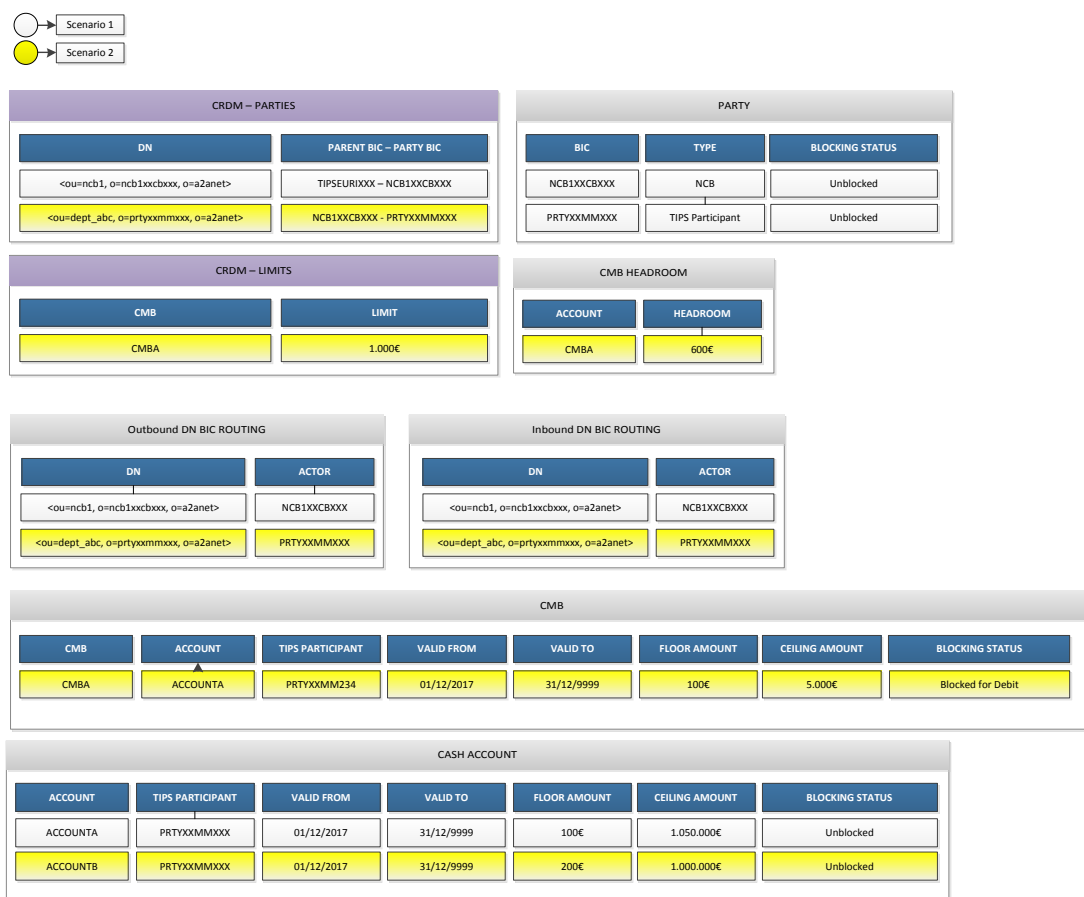
Figure 127126 – Reference Data Management examples: data constellation
