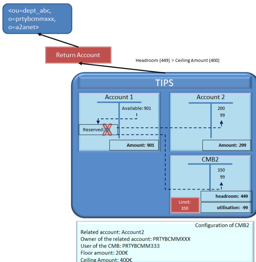
Figure 9998 – Ceiling notification settlement
