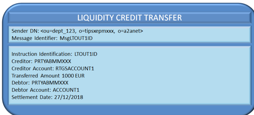
Figure 9190 – Outbound Liquidity Transfer order: forwarding to the RTGS
