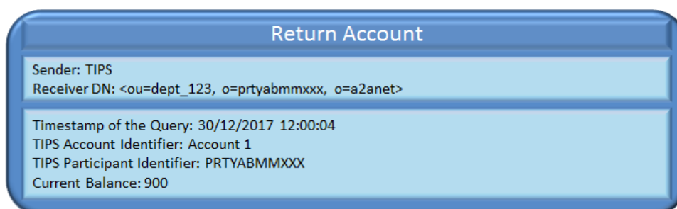
Figure 9897 – Floor notification ReturnAccount
