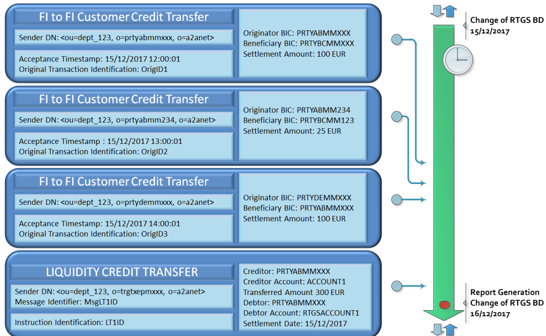
Figure 113112 – Statement of Account Turnover example: list of transactions
