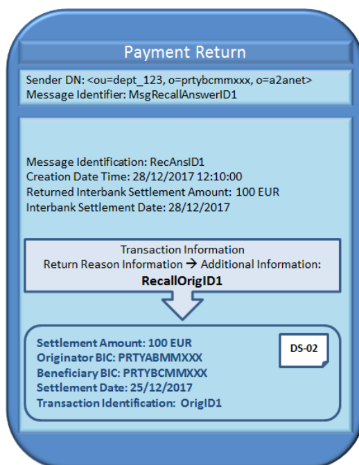
Figure 61 – Recall unsuccessful scenario: Duplicate check failed – PaymentReturn
