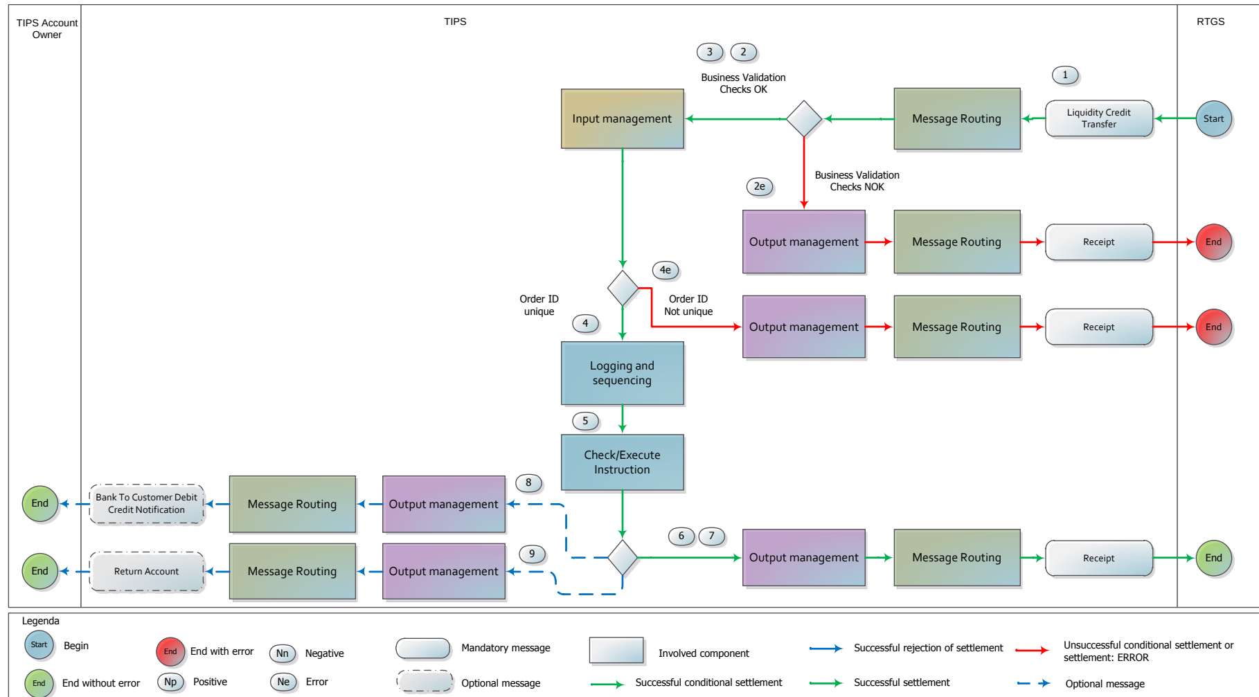
Figure 7170 – Inbound Liquidity Transfer Order flow
