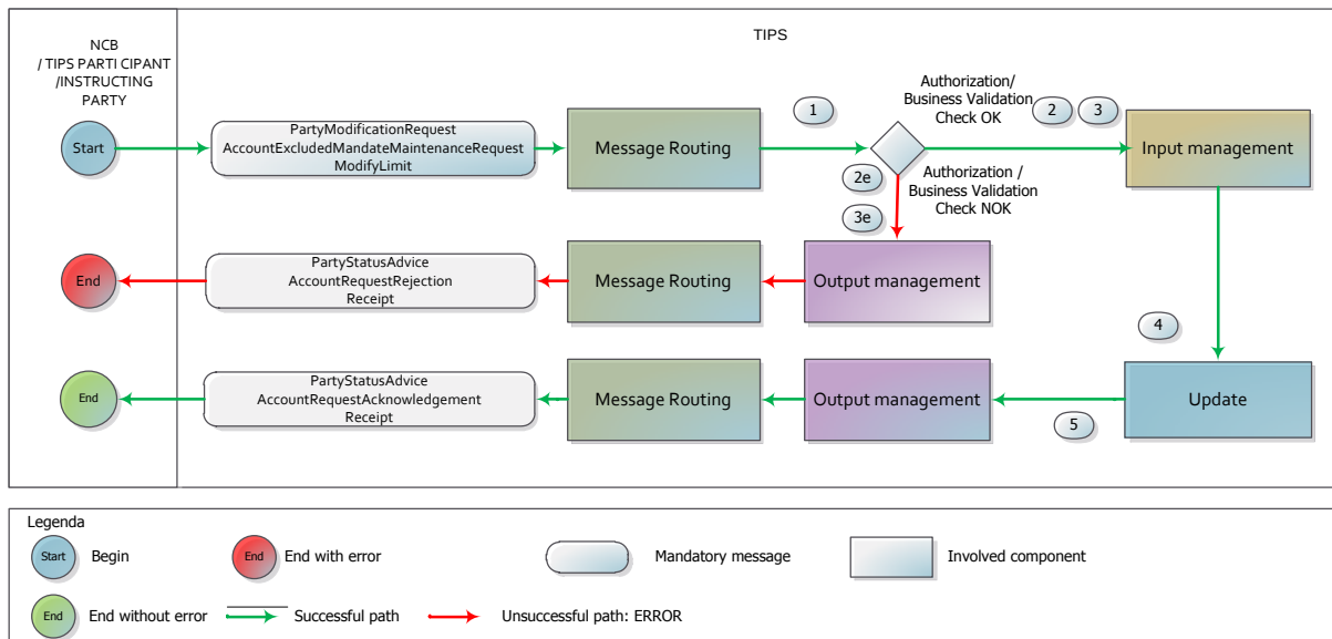
Figure 126125 – Reference Data Messages flow
