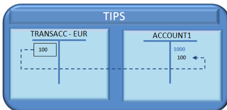
Figure 7473 – Successful Inbound Liquidity Transfer order settlement
