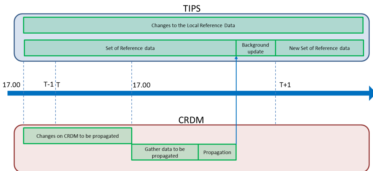
Figure 13 – Interaction between CRDM and TIPS 13
