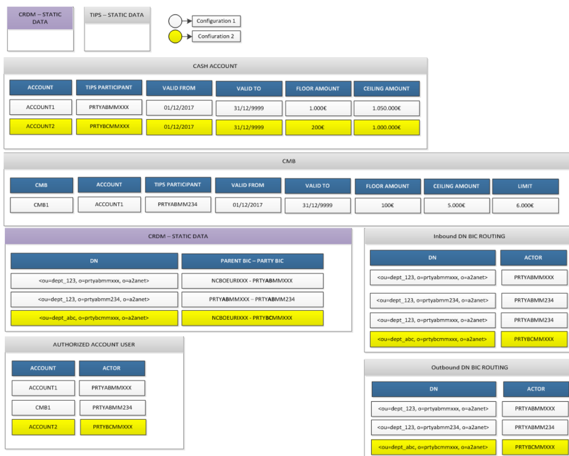
Figure 102101 – Queries examples: data constellation
