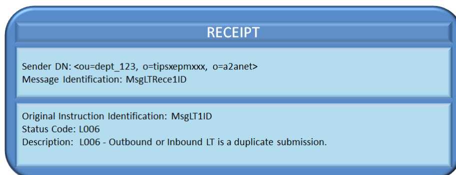
Figure 7978 – Unsuccessful Inbound Liquidity Transfer order Receipt
