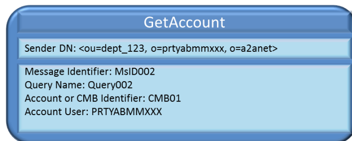
Figure 105104 – Successful Get Account
