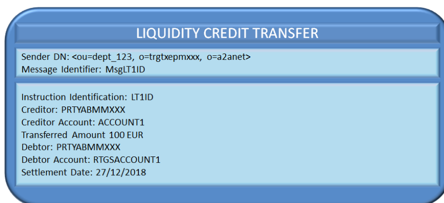
Figure 7372 – Successful Inbound Liquidity Transfer order: liquidity credit transfer
