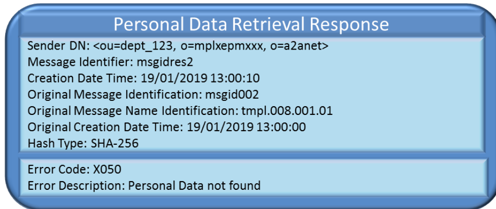
Figure 54 – Unsuccessful scenario 2 – PersonalDataRetrievalResponse
