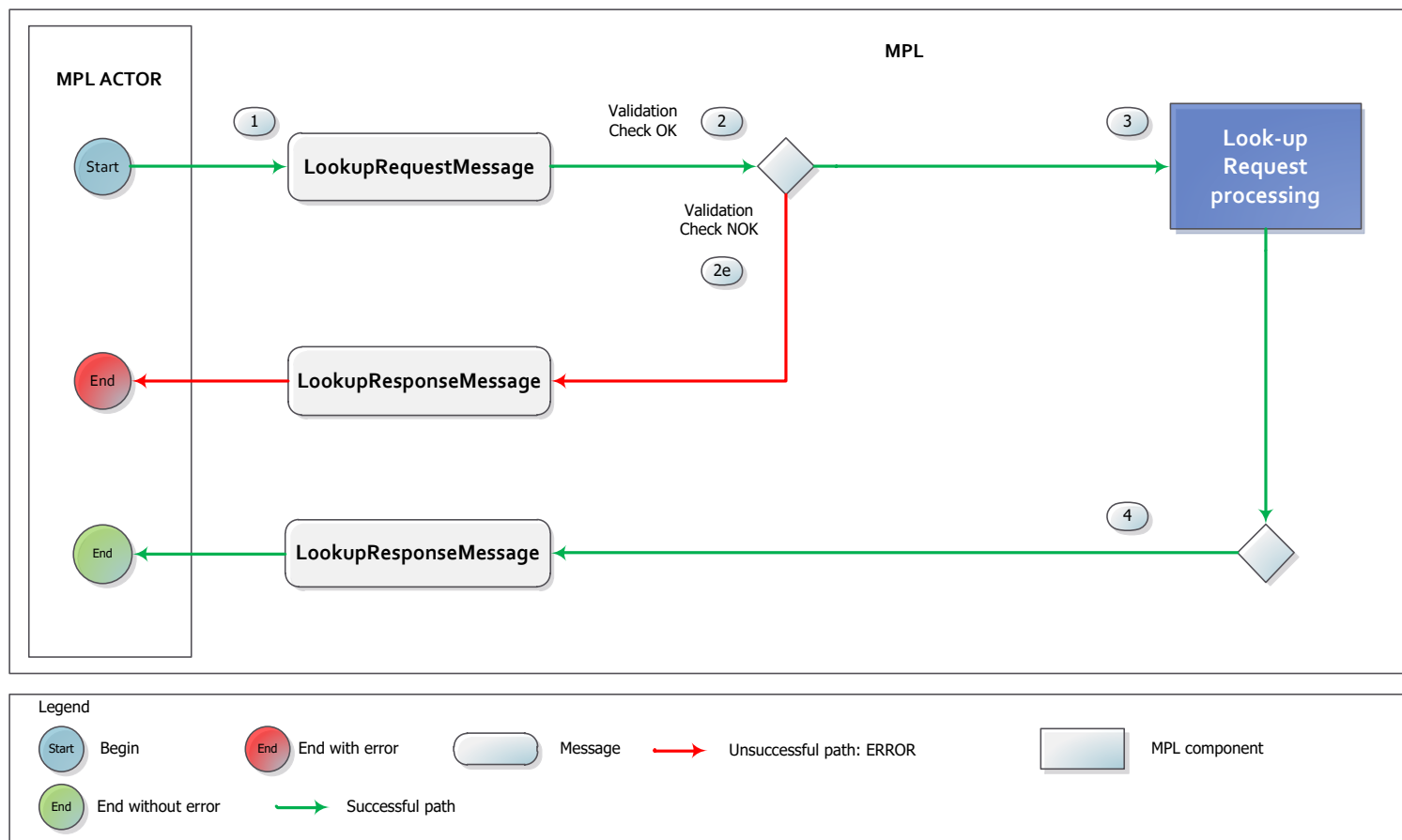
Figure 5 – Look-Up process
