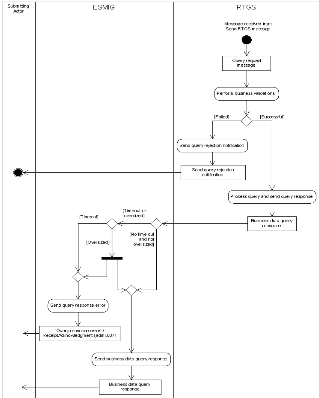
Figure 109: Send RTGS query
