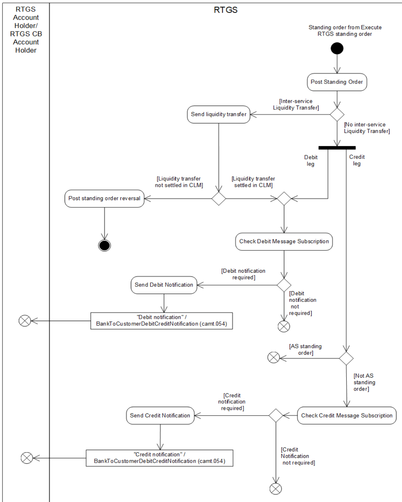
Figure 65: Settle standing order in RTGS
