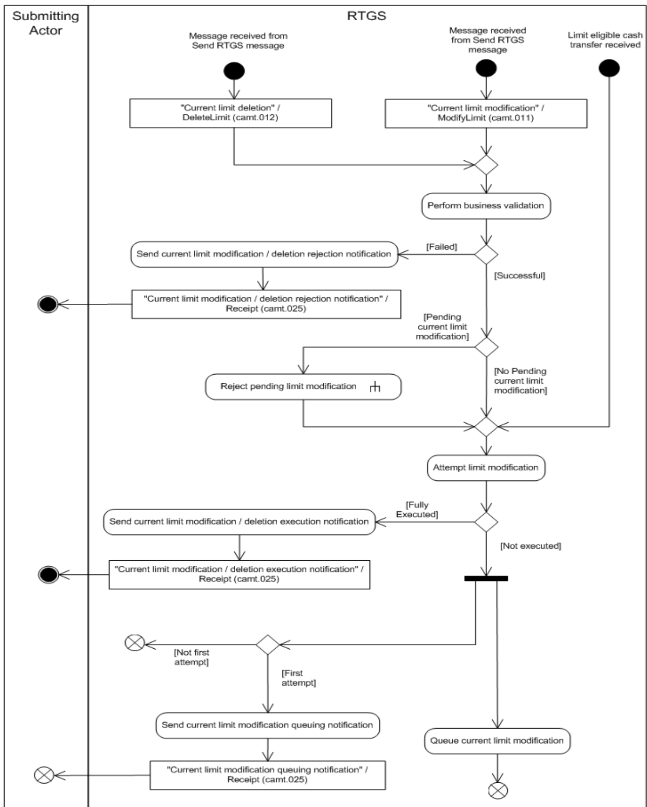
Figure 102: Modify current limit
