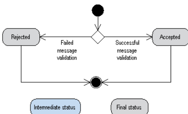
Figure 47: RTGS inbound message status diagram
