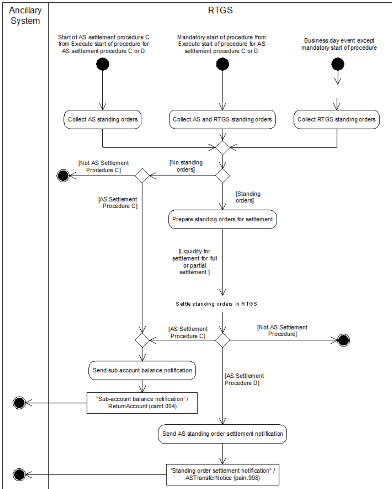
Figure 64: Execute RTGS standing order
