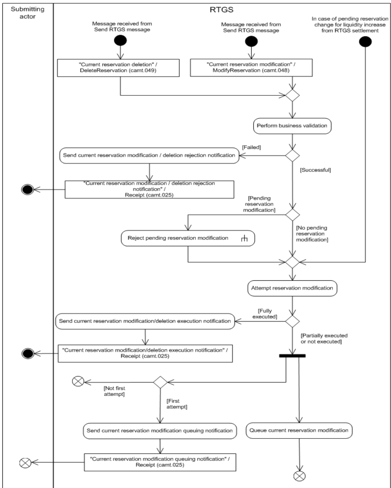
Figure 104: Manage current reservation
