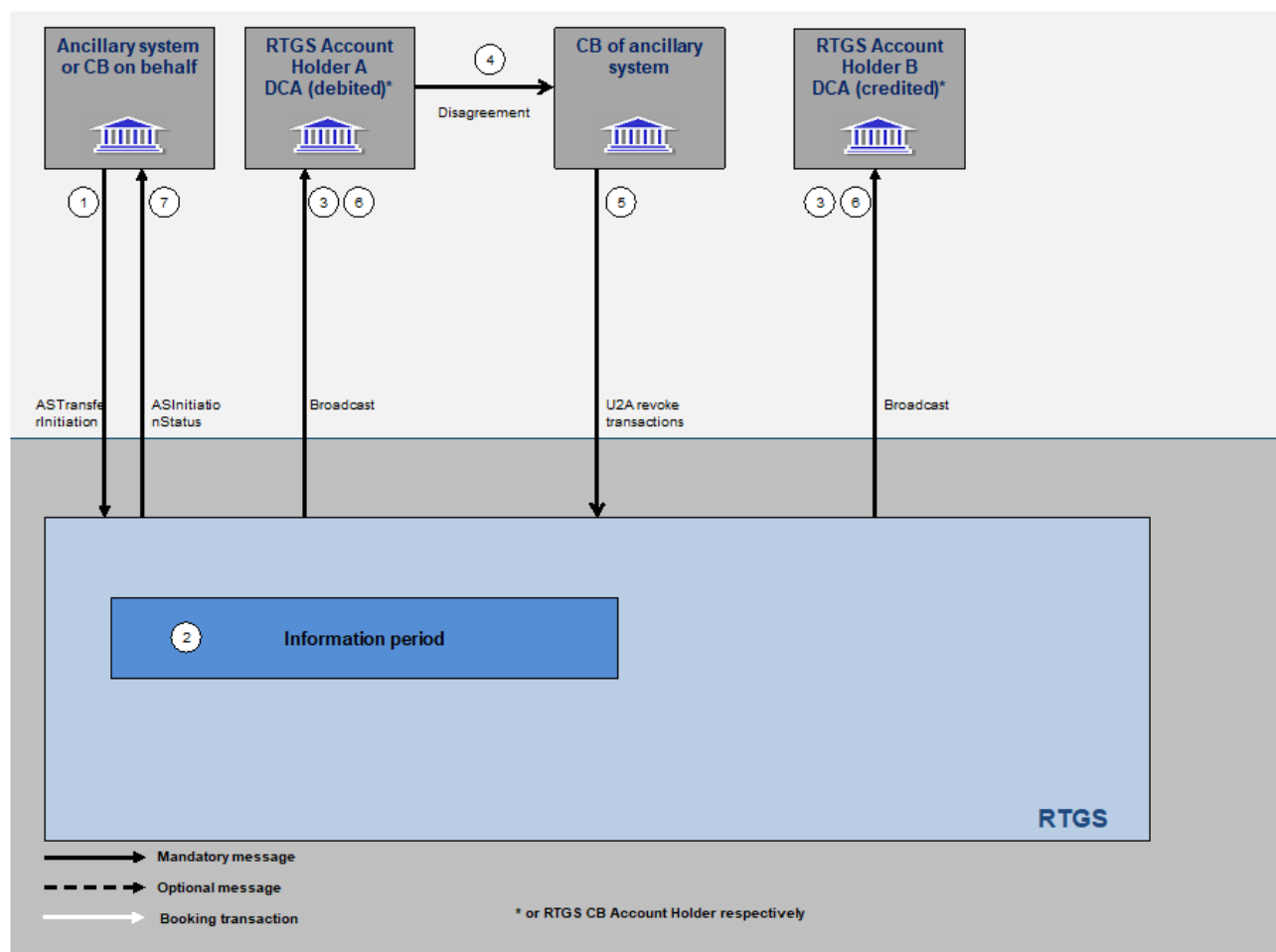
Figure 35: Flow information period
