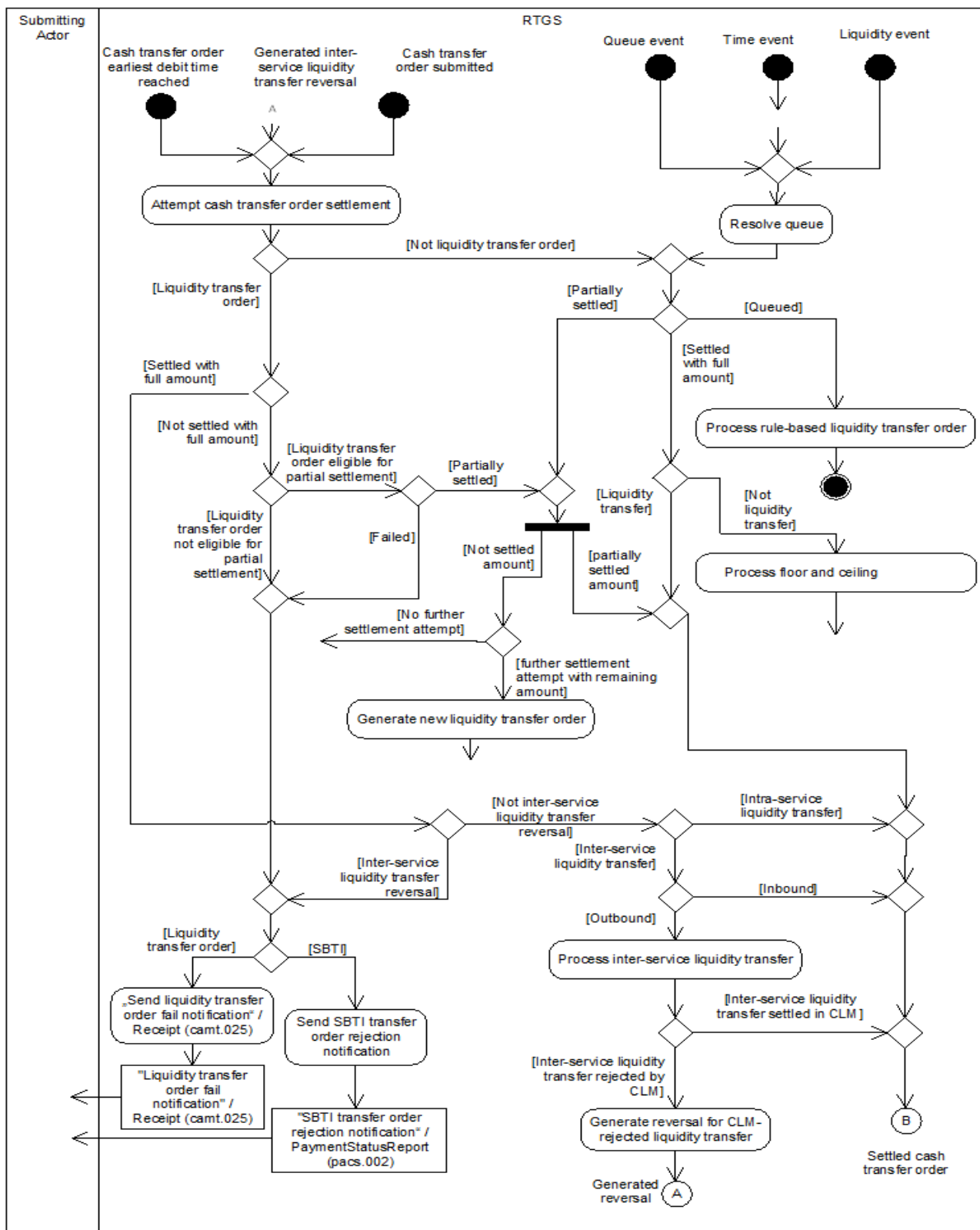
Figure 66: Standard RTGS settlement I
