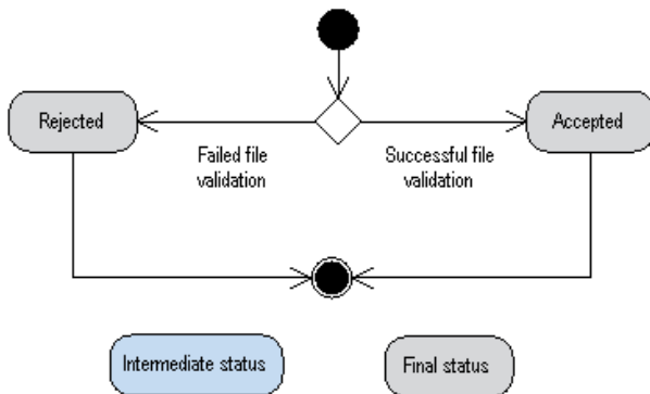
Figure 46: RTGS inbound file status diagram
