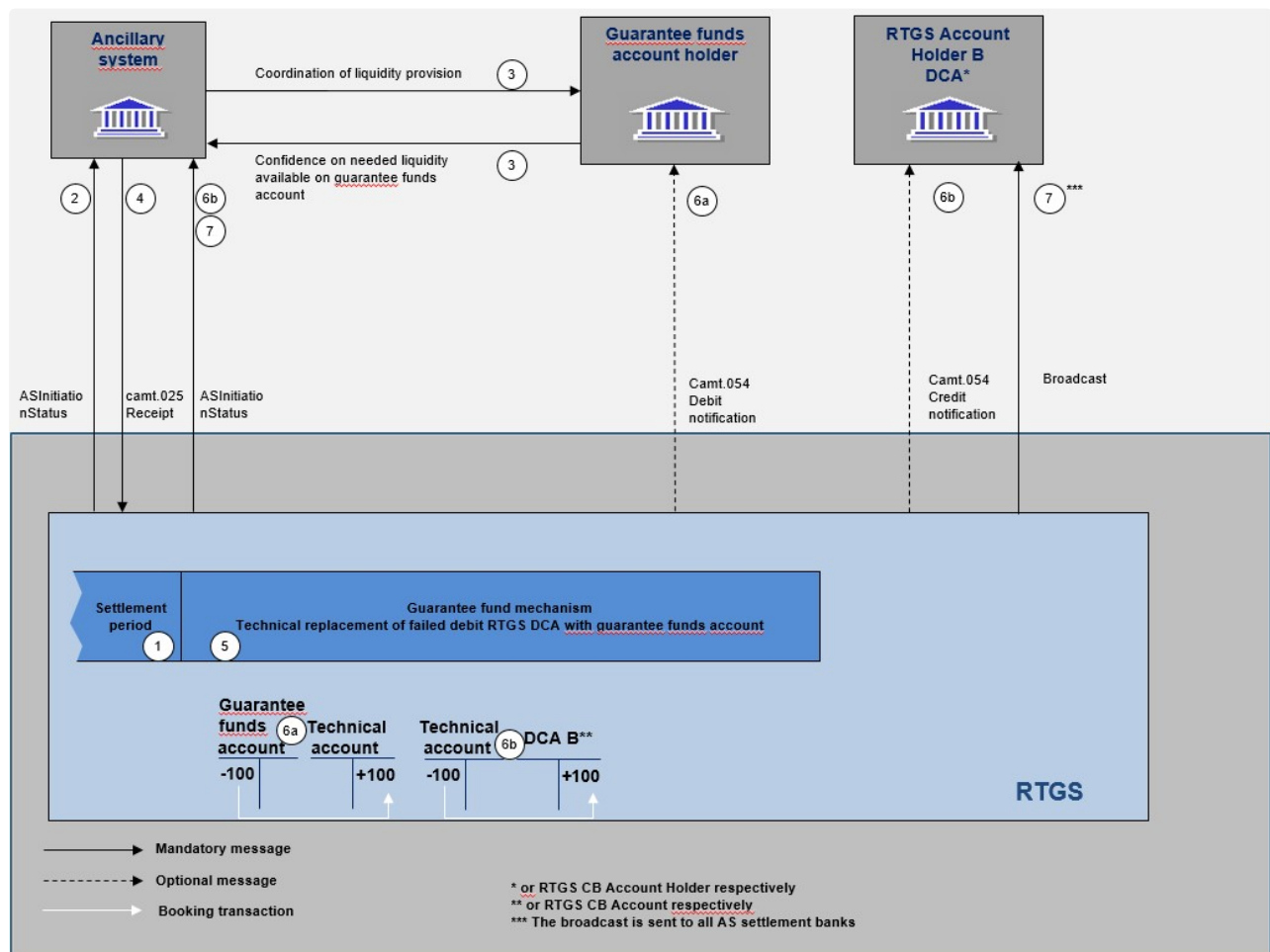
Figure 36: Flow guarantee fund mechanism
