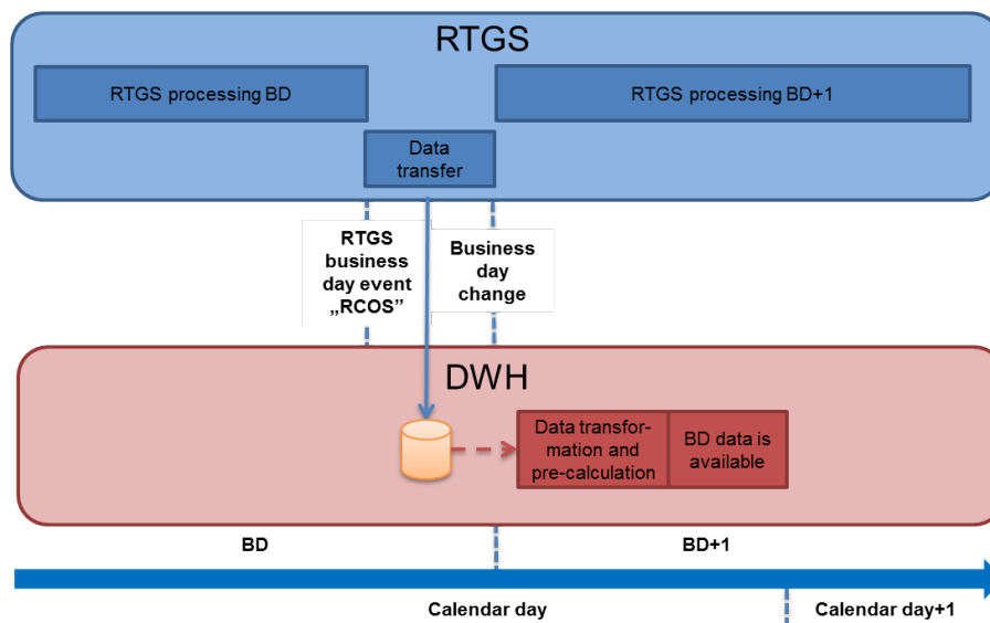
Figure 54: Interaction between RTGS and DWH
