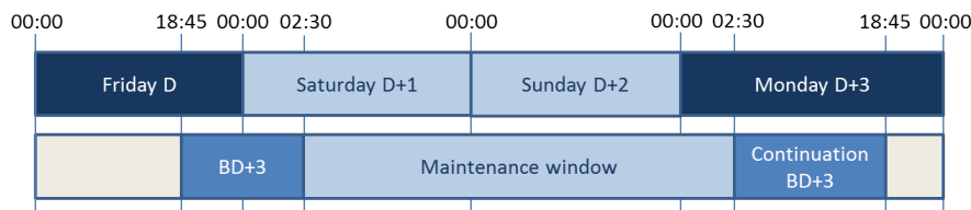
Figure 13: Saturday and Sunday as T2 closing days
