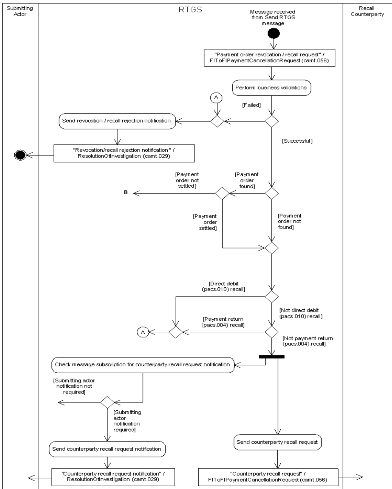
Figure 60: Request payment order revocation or recall I
