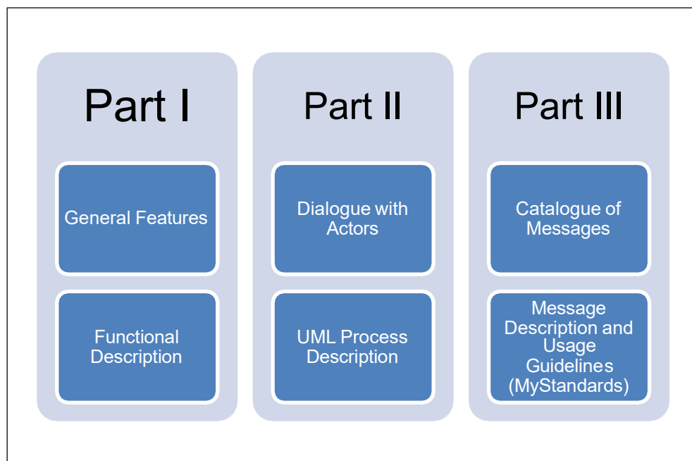
Figure 1 - UDFS Structure
