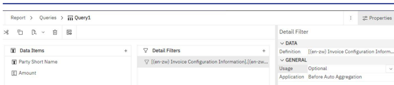
Figure 430 - Create a Prompt Directly in a Report Page
