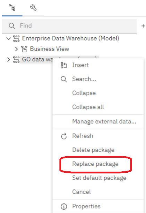
Figure 390 - Adding data - Add a source - Right click item - Replace package
