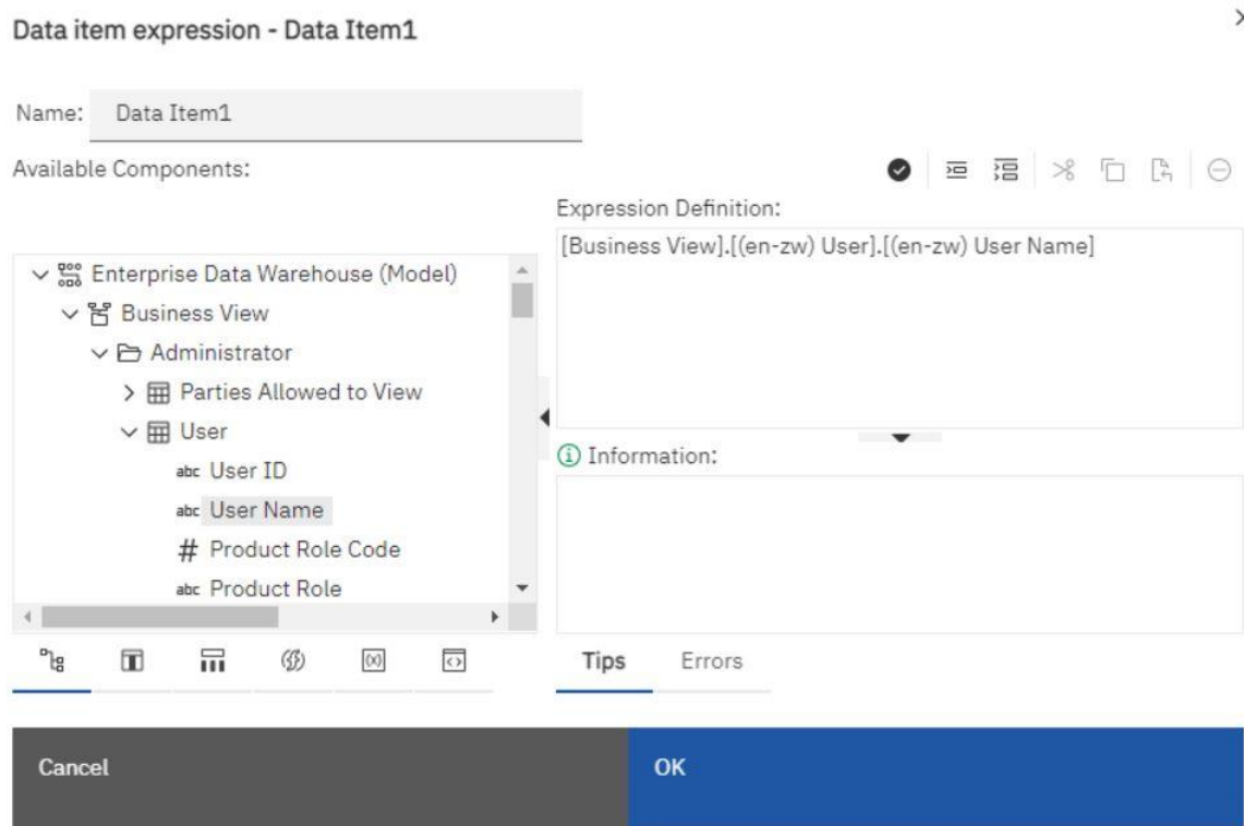
Figure 364 - Insert a Query Calculation - Specify Query Calculation - Data items
