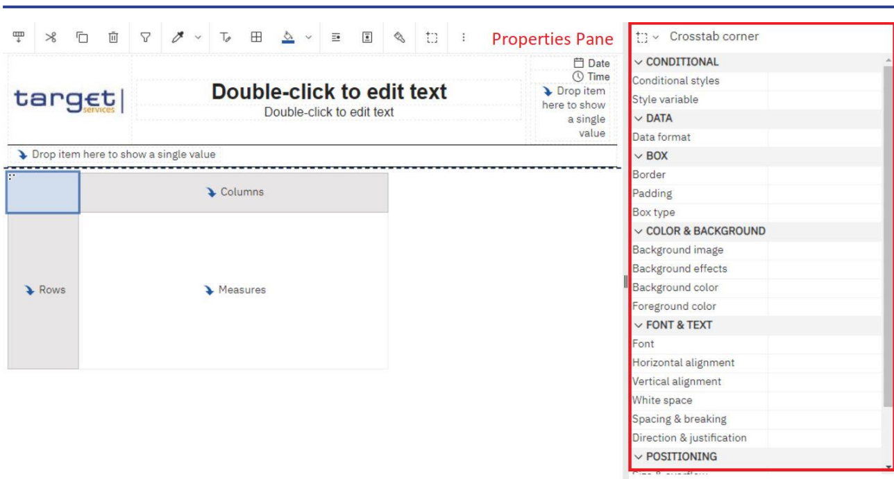
Figure 336 - Toolbox bar - Properties Pane
