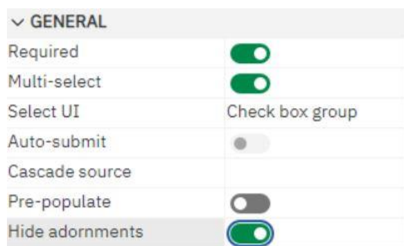
Figure 443 - Modifying prompts - Properties - General - Hide adornments
