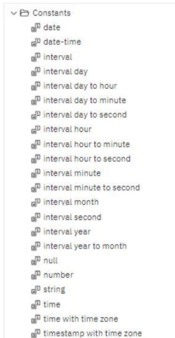
Figure 379 - Insert a Query Calculation - Constants
