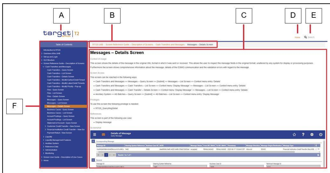
Figure 74 - Online Help
