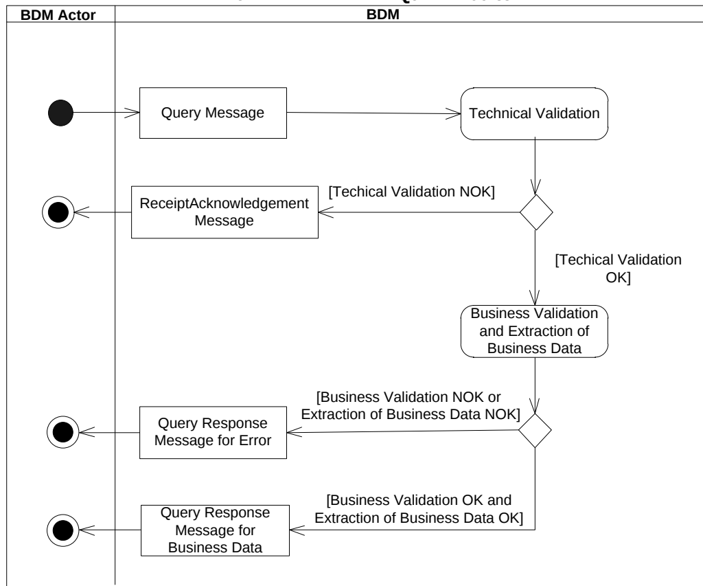
DIAGRAM 14 - BDM DATA QUERY PROCESS
