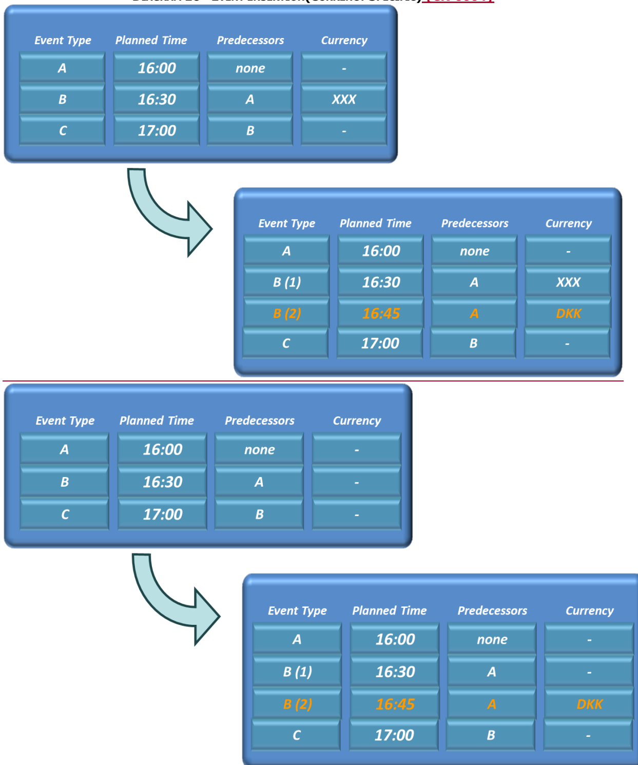
DIAGRAM 10 - EVENT INSERTION(CURRENCY SPECIFIC) {CR-0064}
