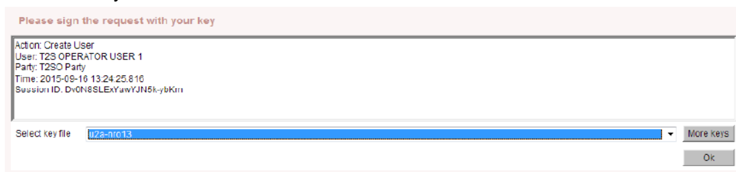
Illustration 18: Digital Signature
