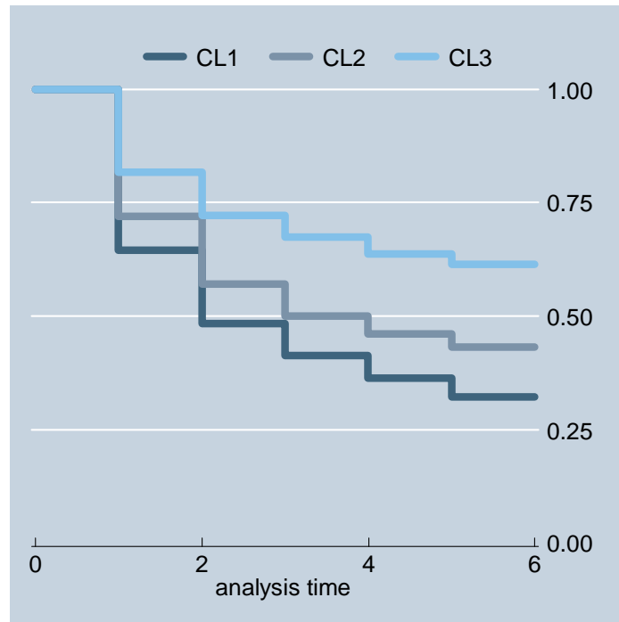
Figure 5. Kaplan-Meier survival estimates by cluster.
