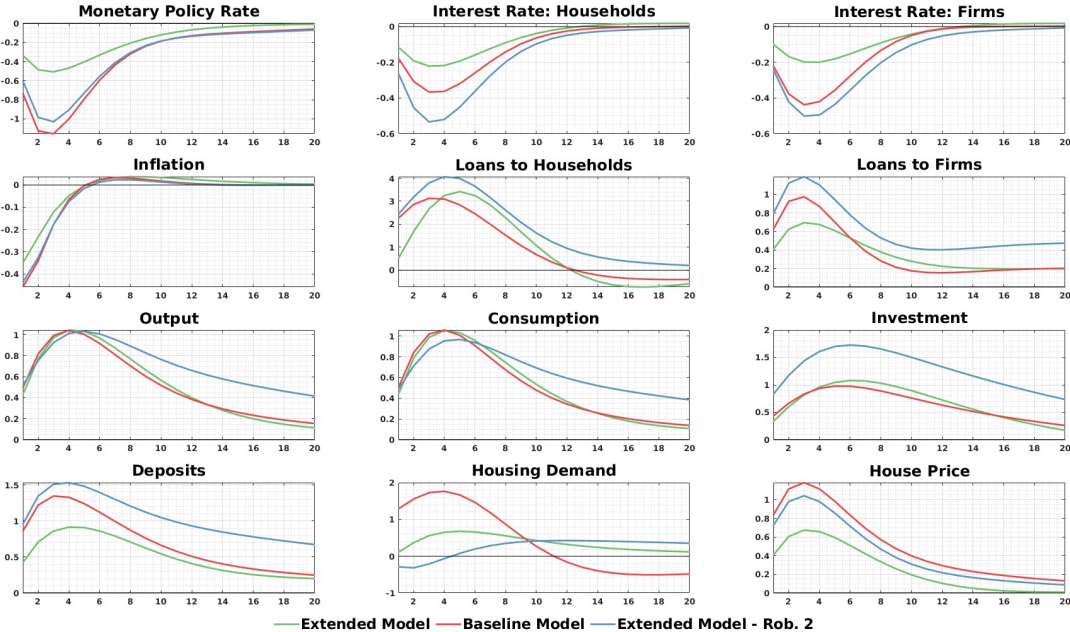
Figure 9. Productivity Shock
