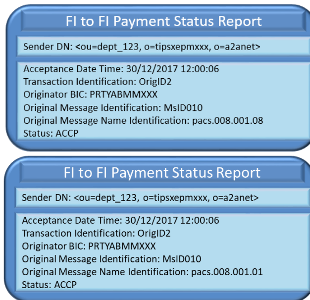
Figure 139 – Successful FIToFIPaymentStatusReport
