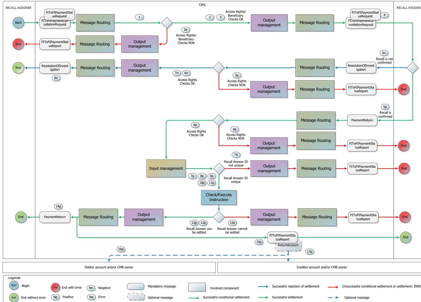
Figure 119 – Recall flow
