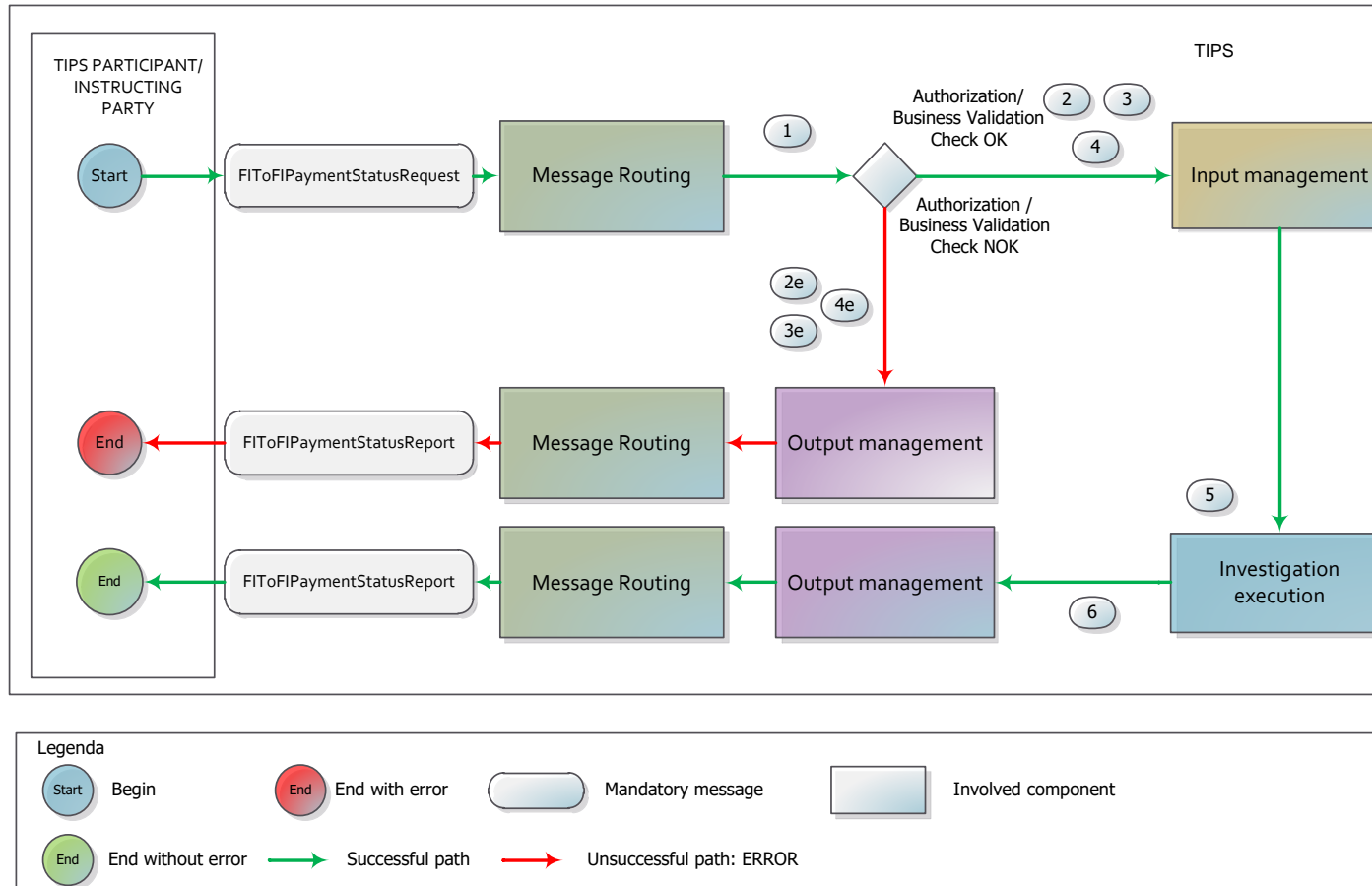
Figure 136 – Investigation Flow
