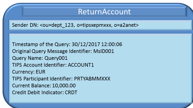
Figure 190 – Successful ReturnAccount
