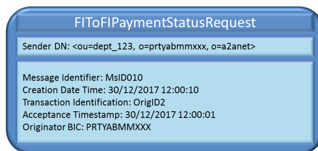
Figure 140 – Unsuccessful FIToFIPaymentStatusRequest
