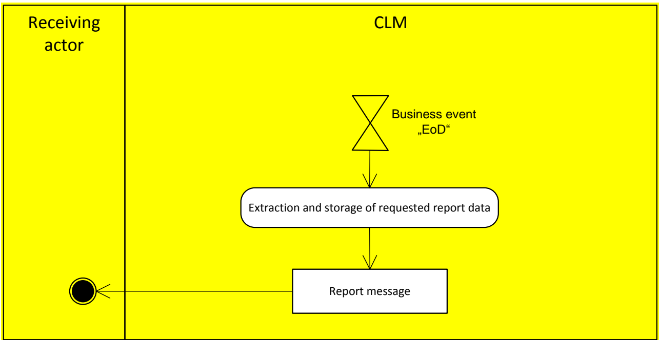
Figure 78 - Receive report
