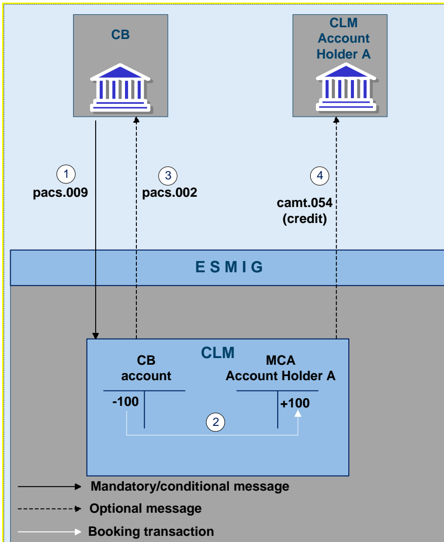
Figure 7 - pacs.009 CBOs
