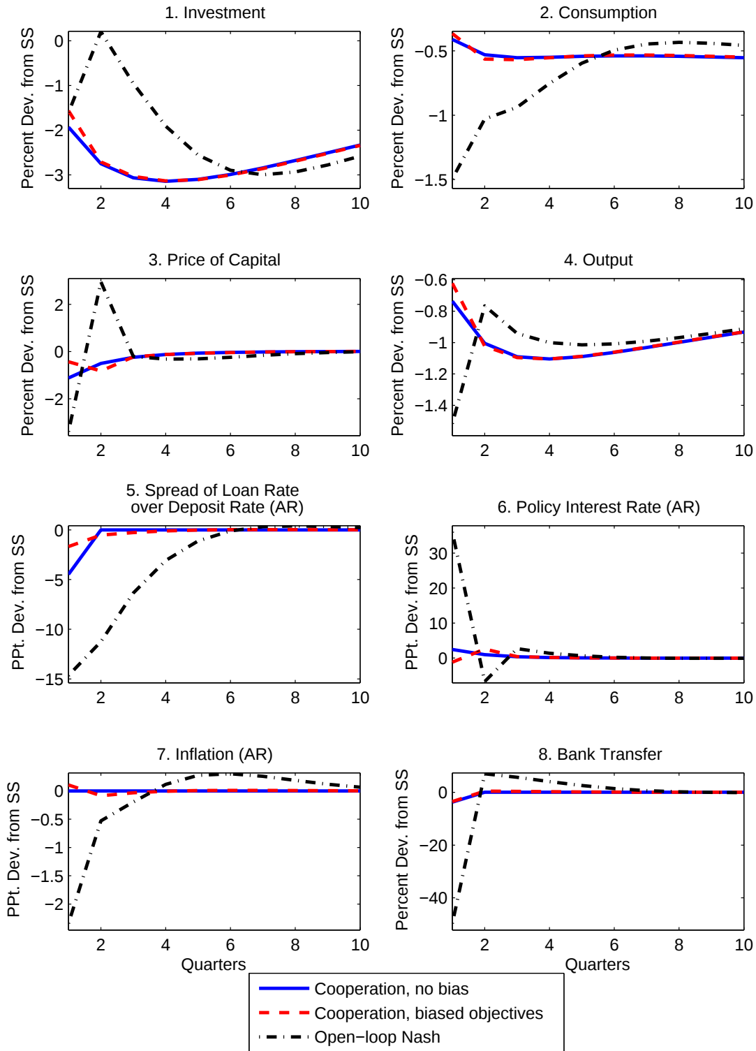
Figure 4: Cooperative and Open-loop Nash Policies in the Macprudential Regulation Model: Responses to a Technology Shock
