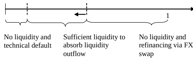
Figure 4: Construction of equilibrium G5. Arrows indicate comparative static reactions to an increase in t (decline in coordination). 19
