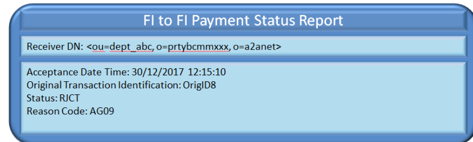
Figure 60 – Delayed Beneficiary-side response: FltoFIPaymentStatusReport
