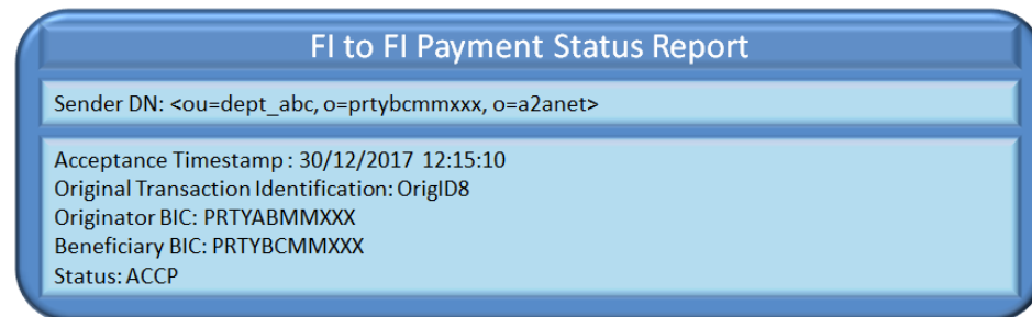
Figure 59 – Delayed Beneficiary-side response: FltoFIPaymentStatusReport
