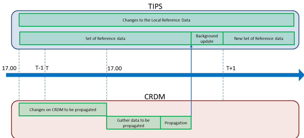
Figure 18 – Interaction between CRDM and TIPS 31
