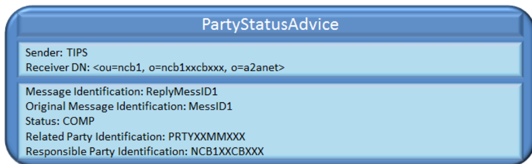
Figure 221 – Successful block of a TIPS Participant: PartyStatusAdvice
